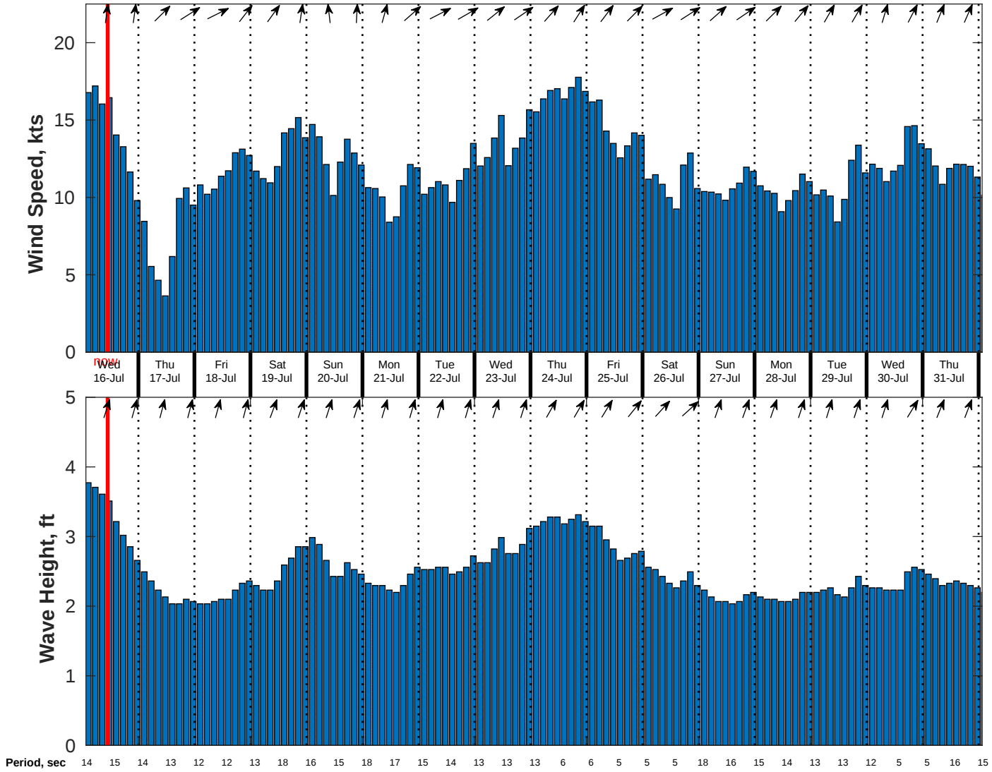
Wind & Wave Forecast for CSA (ONHYM) PPL EBS - Sierra Leone from 15-Jul-2025 01:00:00 to 31-Jul-2025 01:00:00
