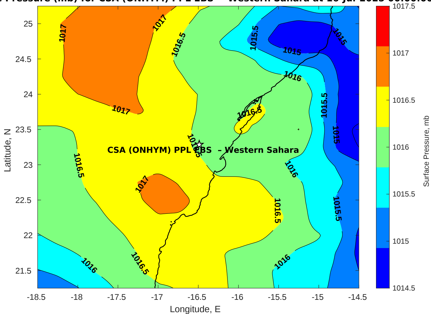
Surface Pressure (mb) for CSA (ONHYM) PPL EBS - Western Sahara at 16-Jul-2025 00:00:00
