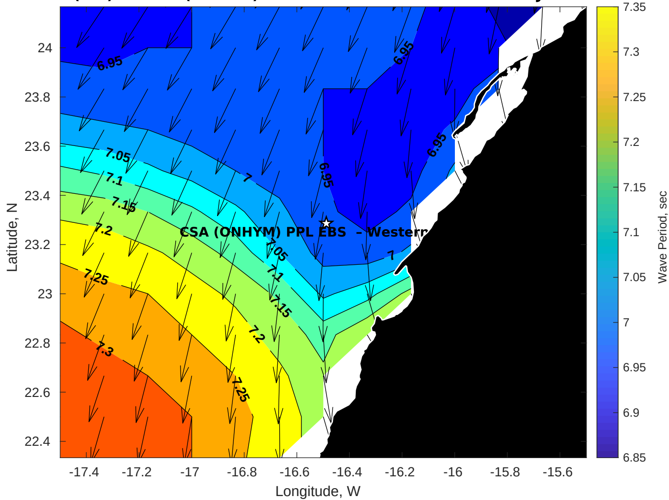
Wave Period (sec) for CSA (ONHYM) PPL EBS - Western Sahara at 15-Jul-2025 09:00:00
