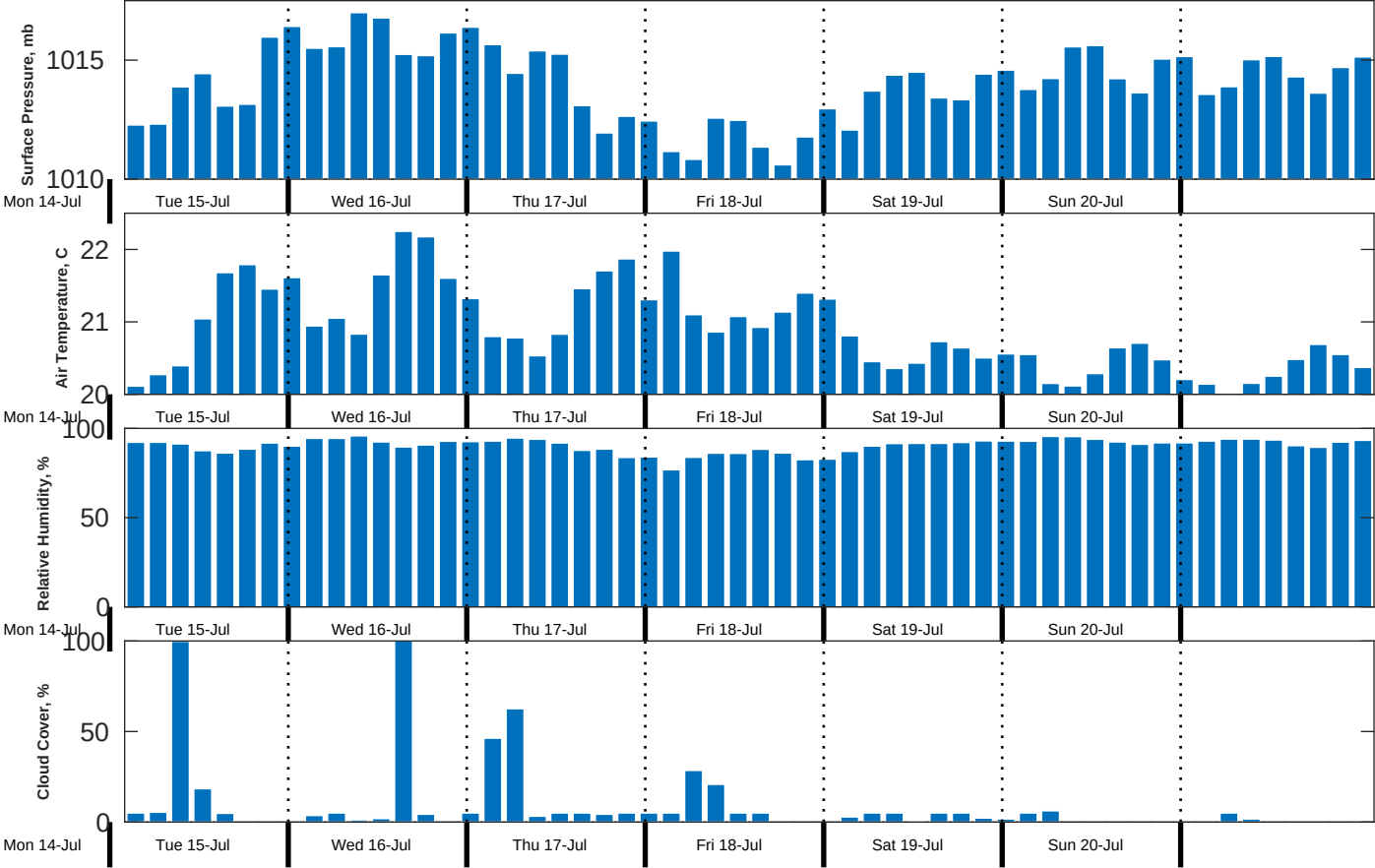
Met Forecast for CSA (ONHYM) PPL EBS - Western Sahara from 15-Jul-2025 00:00:00 to 22-Jul-2025 00:00:00
