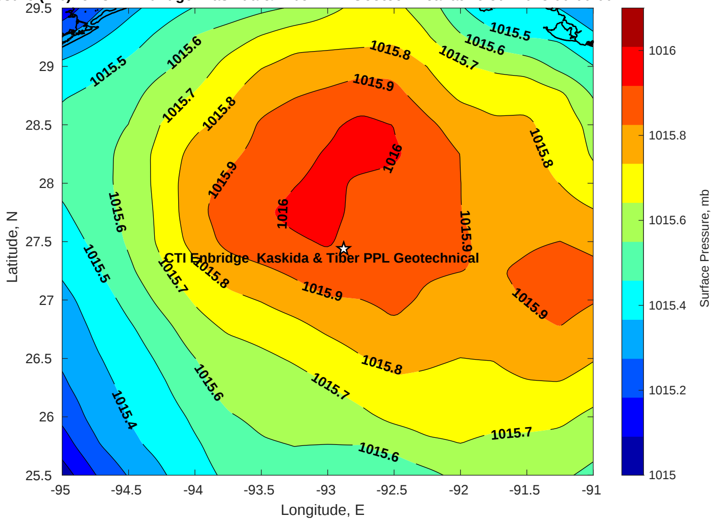
Surface Pressure (mb) for CTI Enbridge Kaskida & Tiber PPL Geotechnical at 16-Jul-2025 00:00:00
