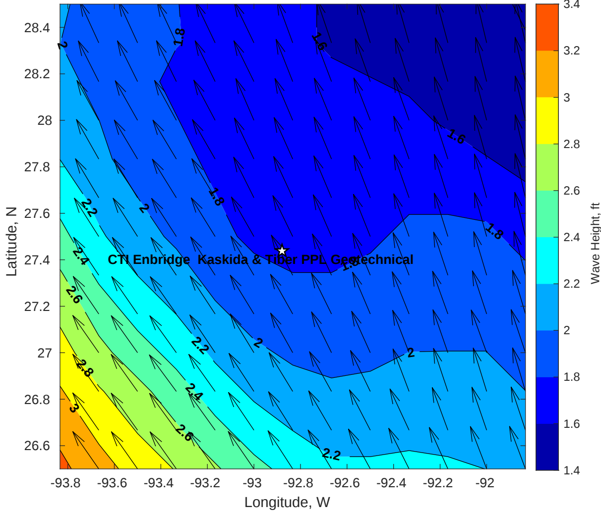
Wave Height (ft) for CTI Enbridge Kaskida & Tiber PPL Geotechnical at 15-Jul-2025 09:00:00
