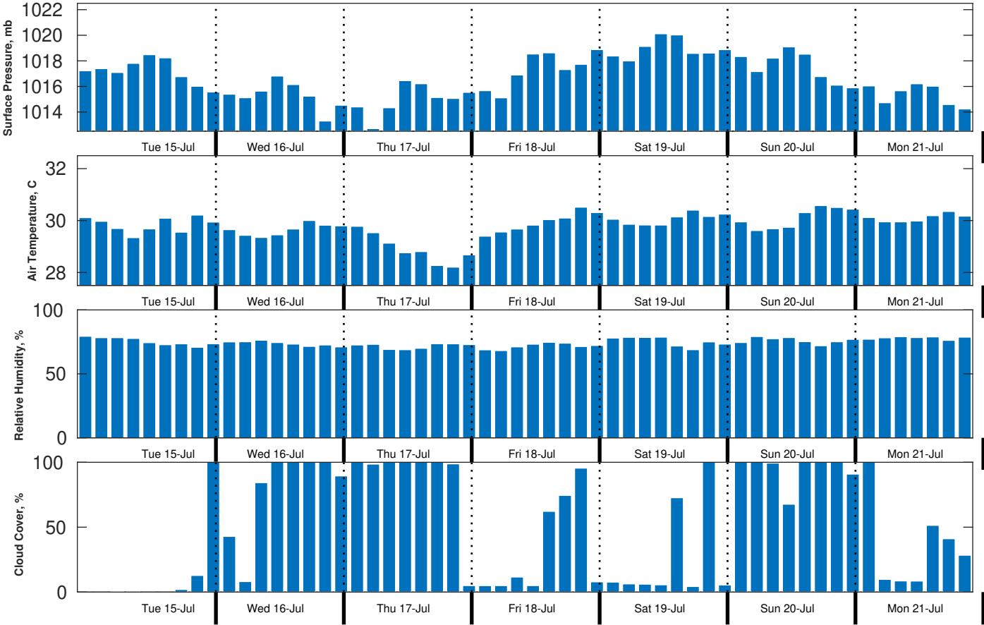
Met Forecast for CTI Enbridge Kaskida & Tiber PPL Geotechnical from 15-Jul-2025 00:00:00 to 22-Jul-2025 00:00:00
