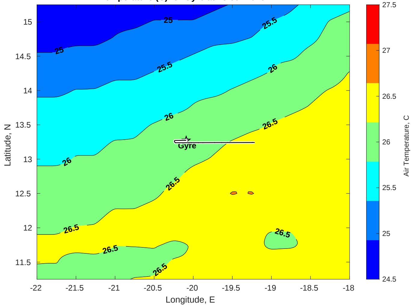
Air Temperature (C) for Gyre at 15-Jul-2025
