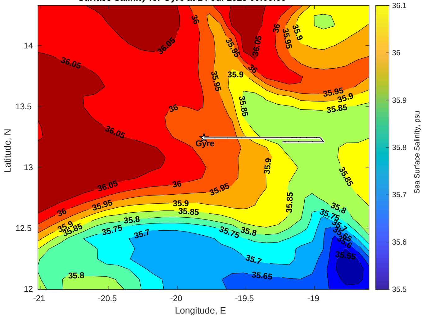
Surface Salinity for Gyre at 14-Jul-2025 00:00:00
