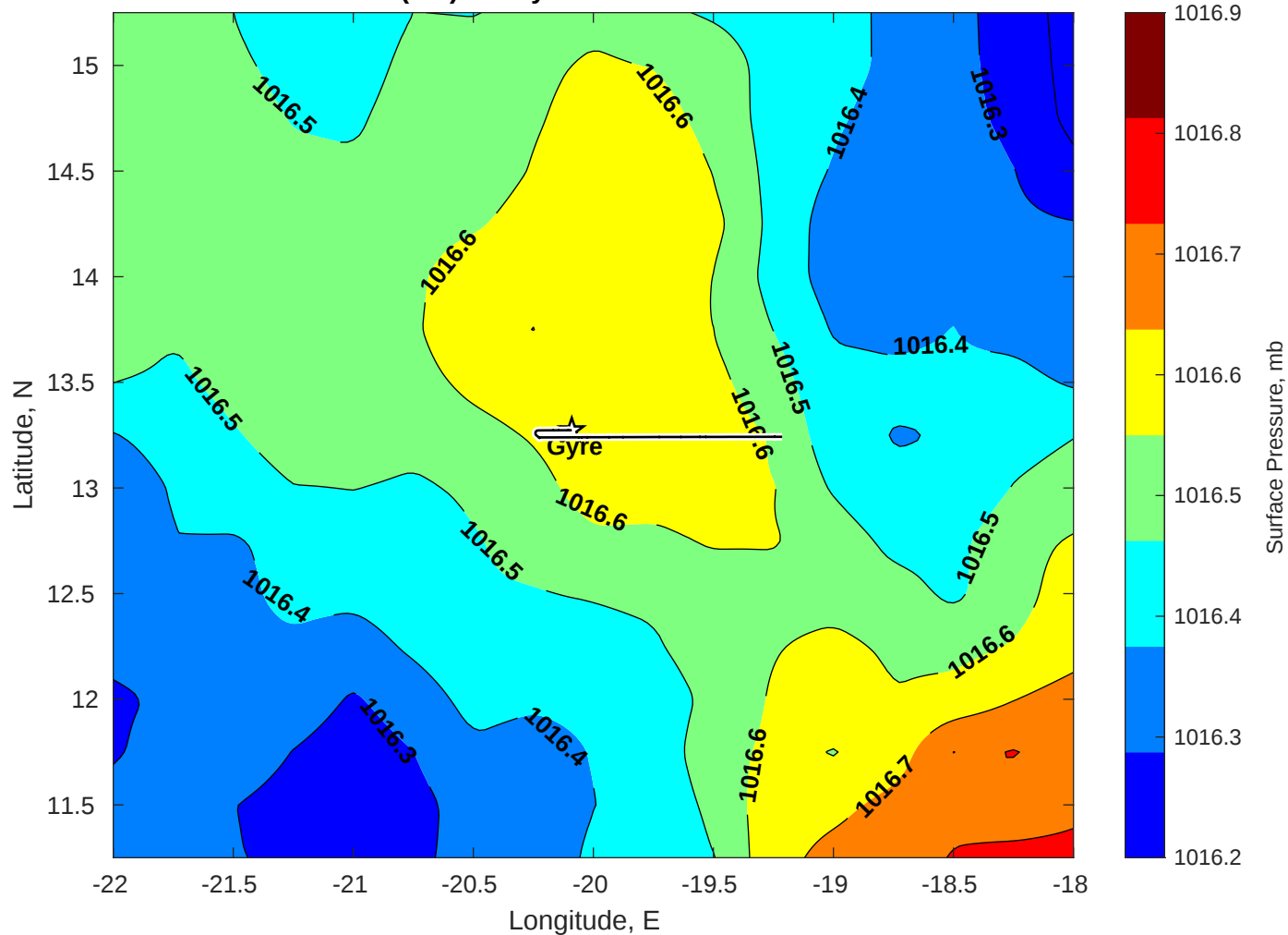
Surface Pressure (mb) for Gyre at 16-Jul-2025 00:00:00
