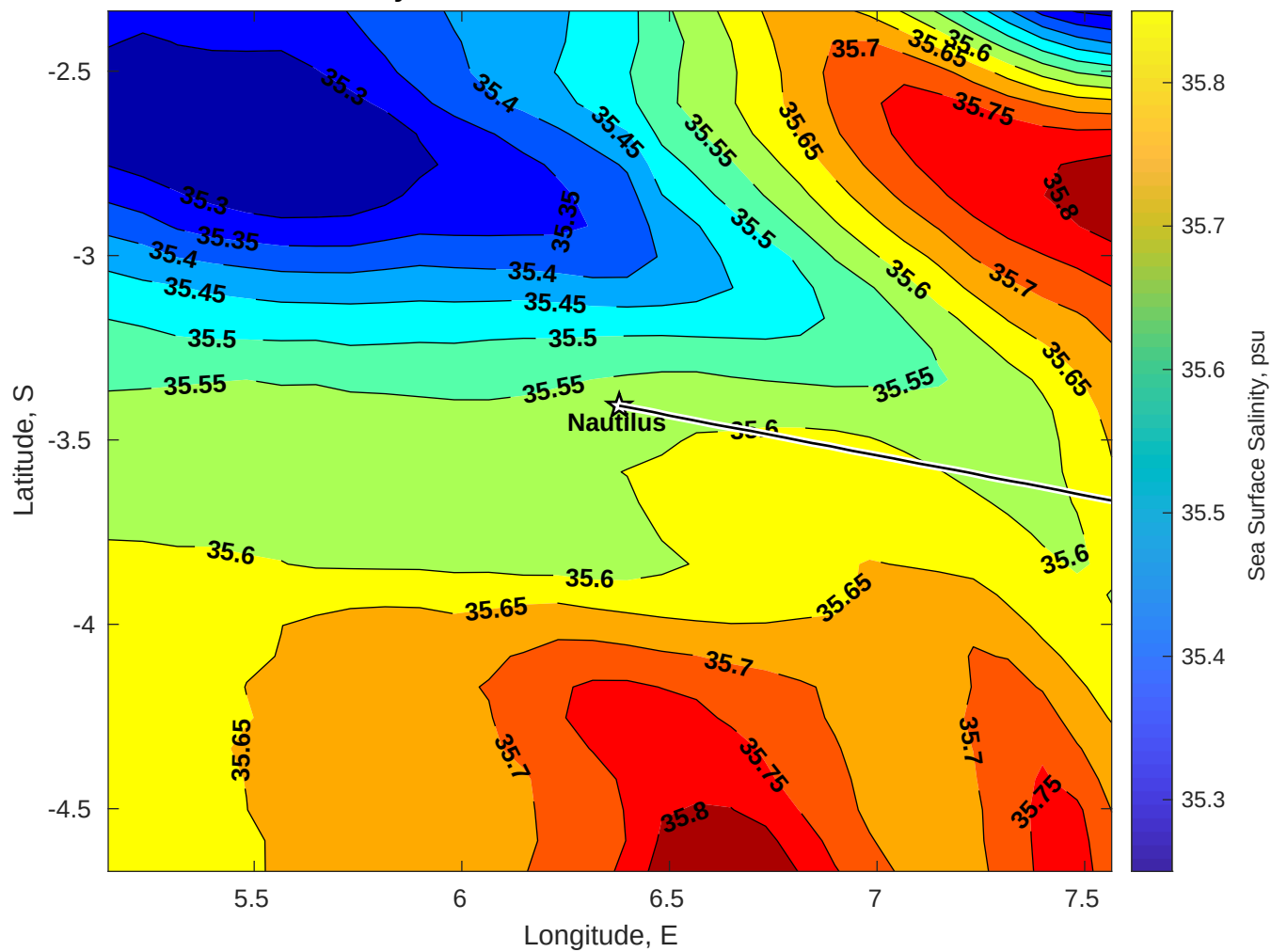
Surface Salinity for Nautilus at 14-Jul-2025 00:00:00
