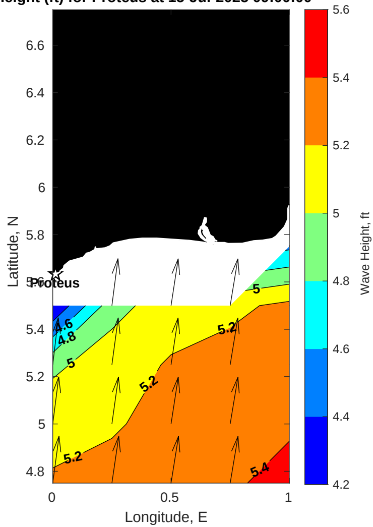
Wave Height (ft) for Proteus at 15-Jul-2025 09:00:00
