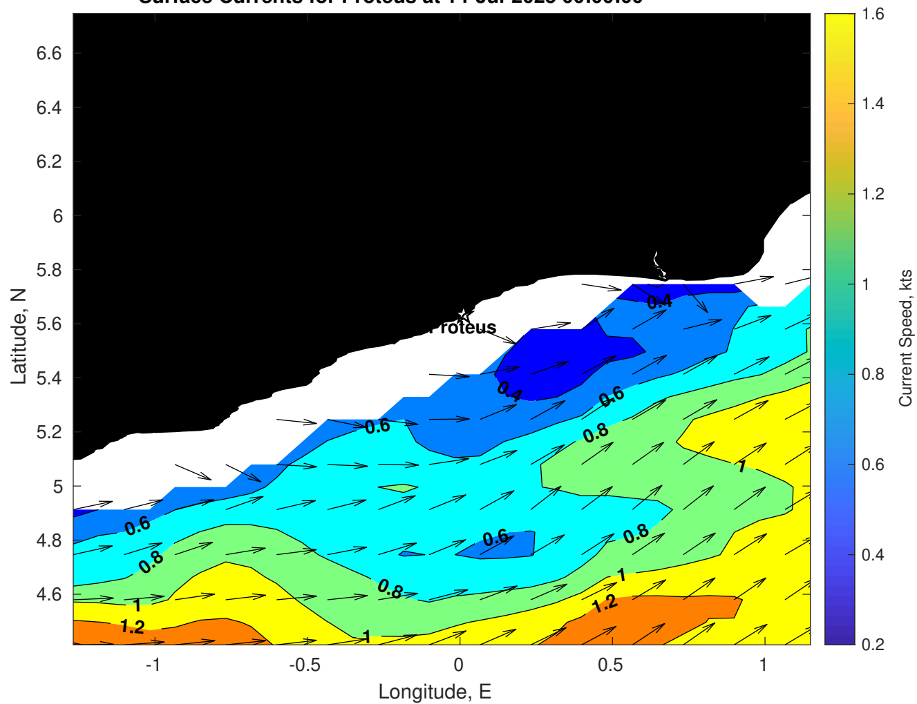
Surface Currents for Proteus at 14-Jul-2025 00:00:00
