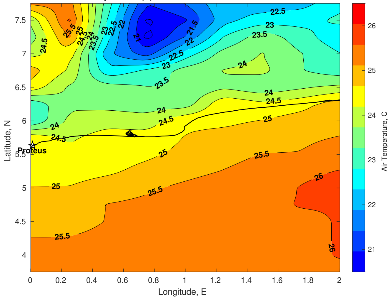
Air Temperature (C) for Proteus at 15-Jul-2025
