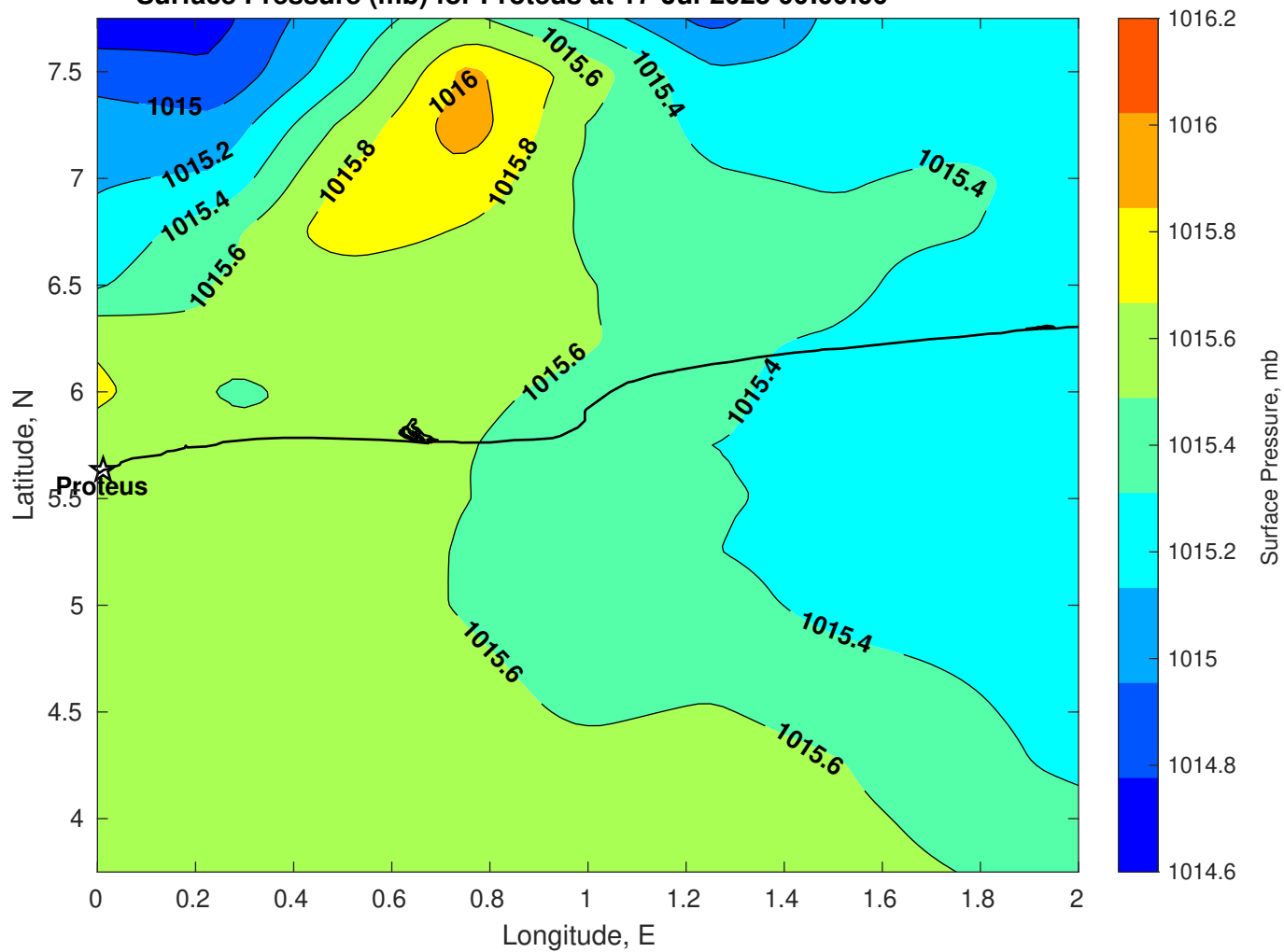
Surface Pressure (mb) for Proteus at 17-Jul-2025 00:00:00
