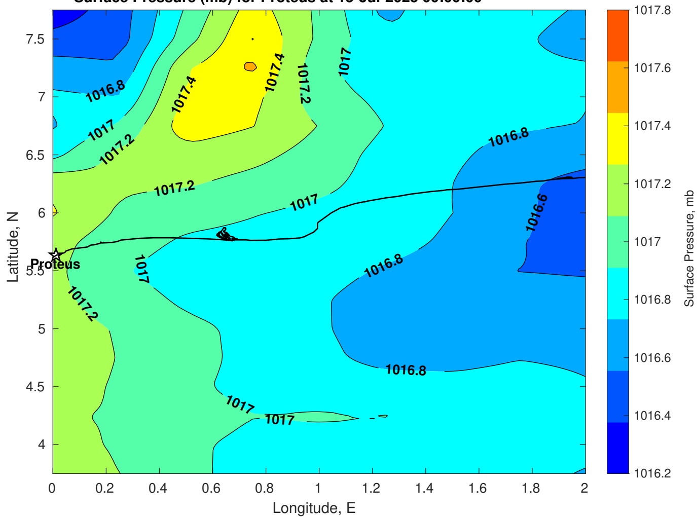
Surface Pressure (mb) for Proteus at 15-Jul-2025 00:00:00
