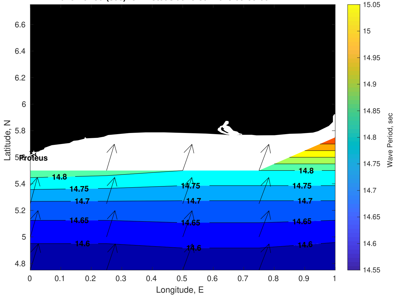
Wave Period (sec) for Proteus at 15-Jul-2025 09:00:00
