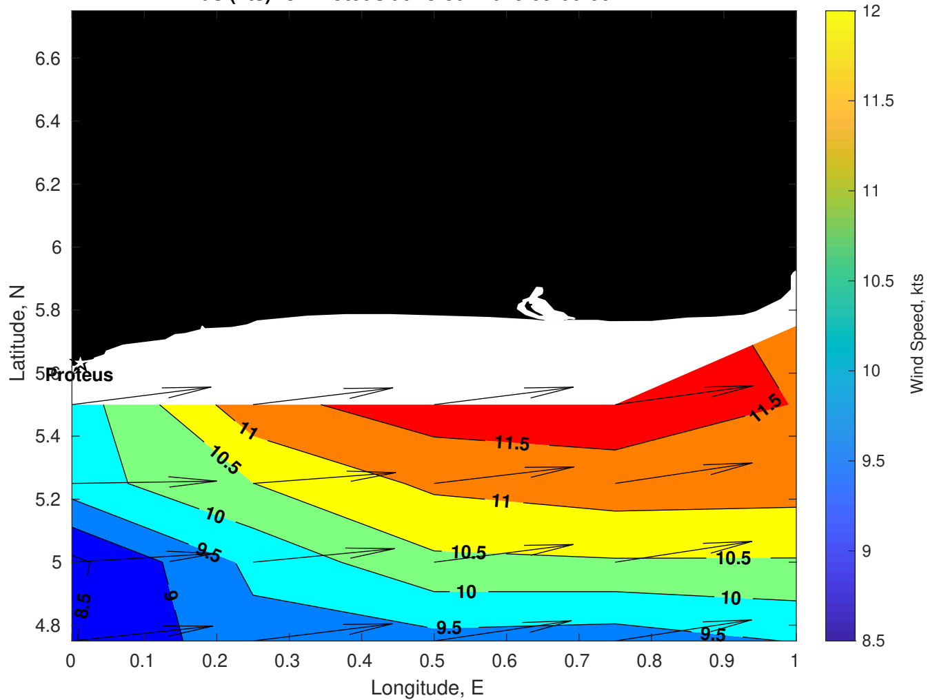
Winds (kts) for Proteus at 15-Jul-2025 09:00:00
