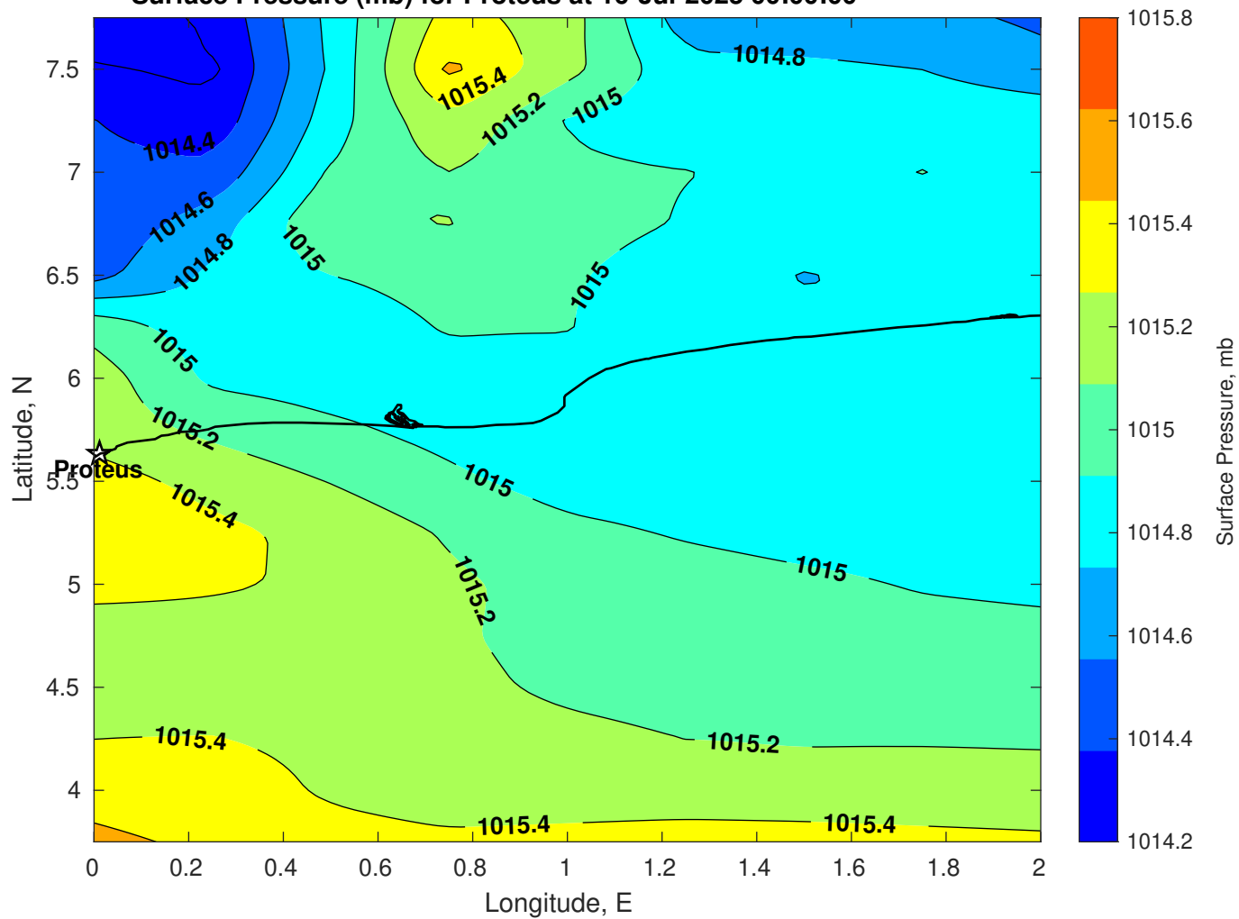
Surface Pressure (mb) for Proteus at 16-Jul-2025 00:00:00
