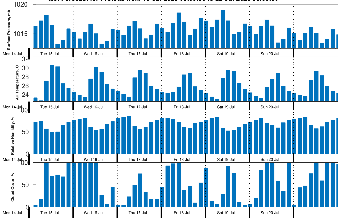
Met Forecast for Proteus from 15-Jul-2025 00:00:00 to 22-Jul-2025 00:00:00
