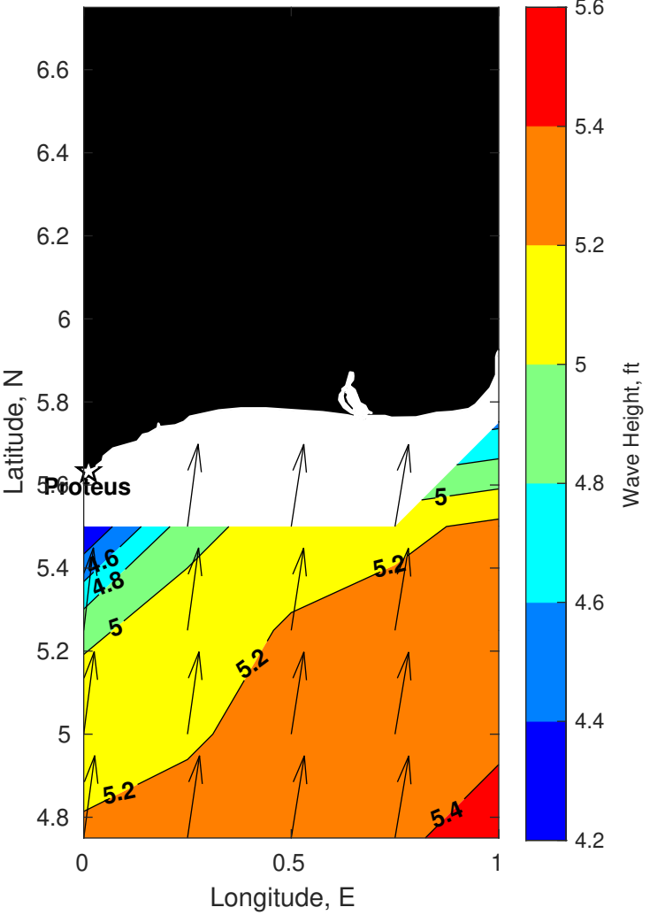
Wave Height (ft) for Proteus at 15-Jul-2025 09:00:00
