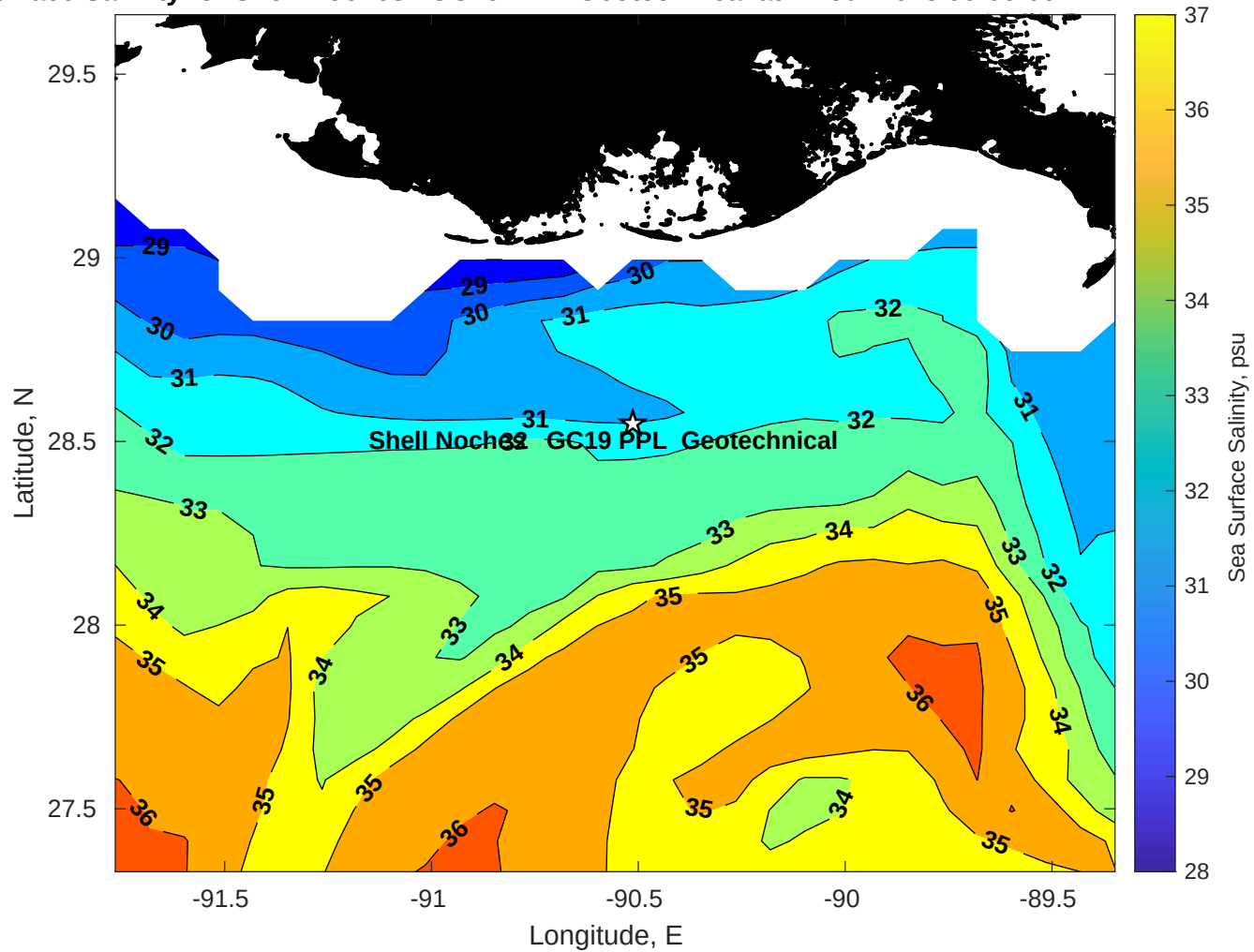
Surface Salinity for Shell Noches GC19 PPL Geotechnical at 14-Jul-2025 00:00:00
