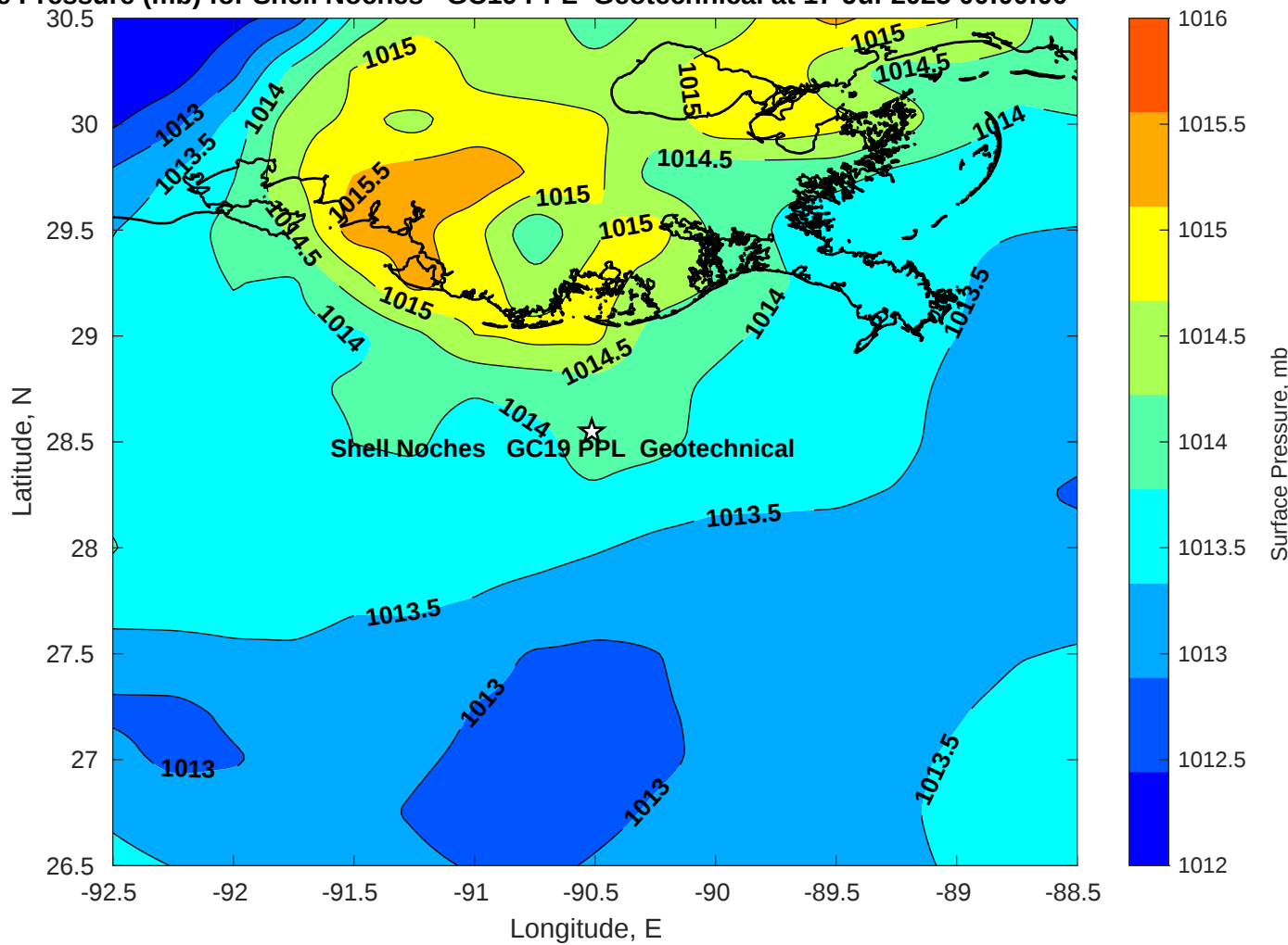
Surface Pressure (mb) for Shell Noches GC19 PPL Geotechnical at 17-Jul-2025 00:00:00
