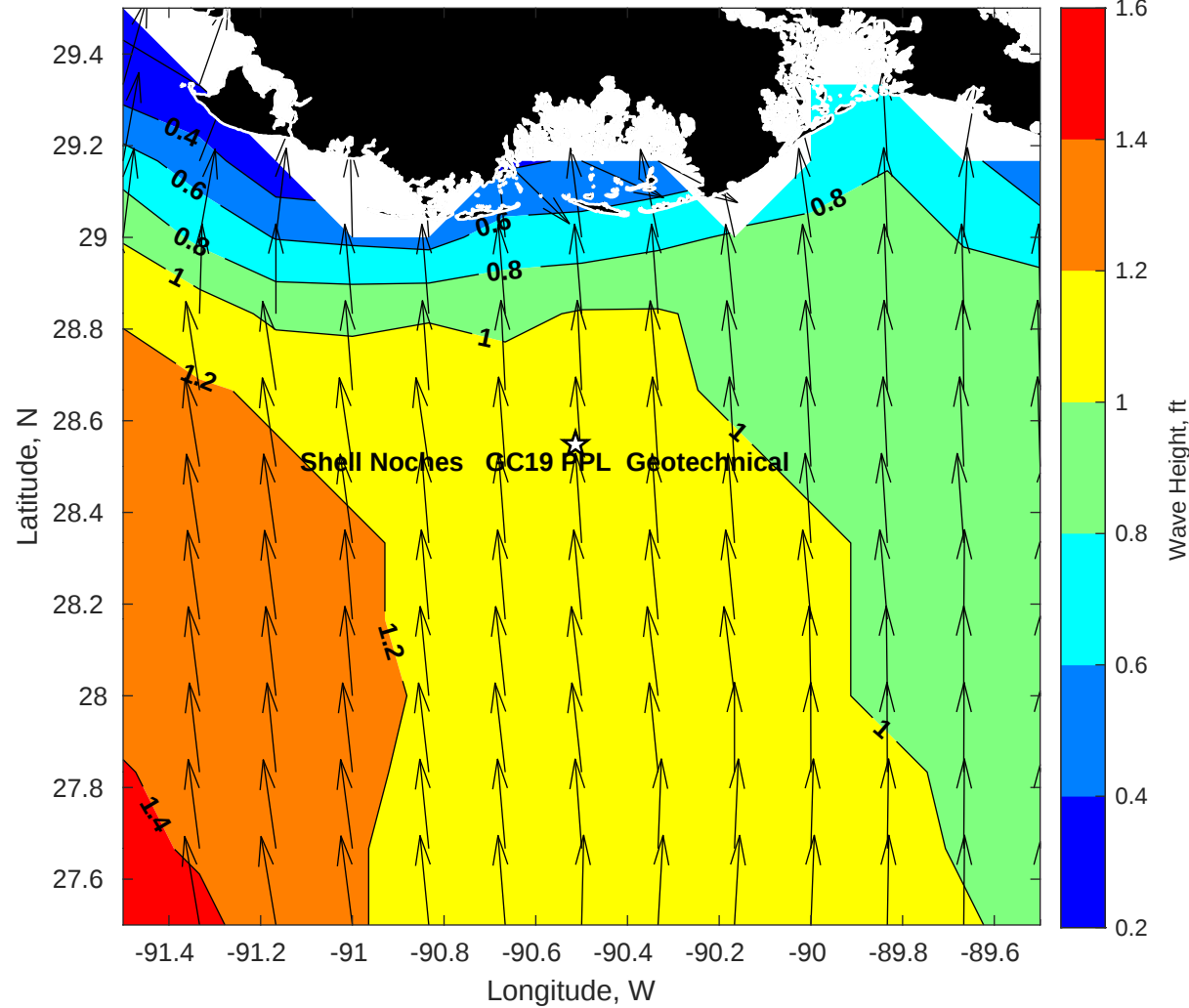
Wave Height (ft) for Shell Noches GC19 PPL Geotechnical at 15-Jul-2025 09:00:00
