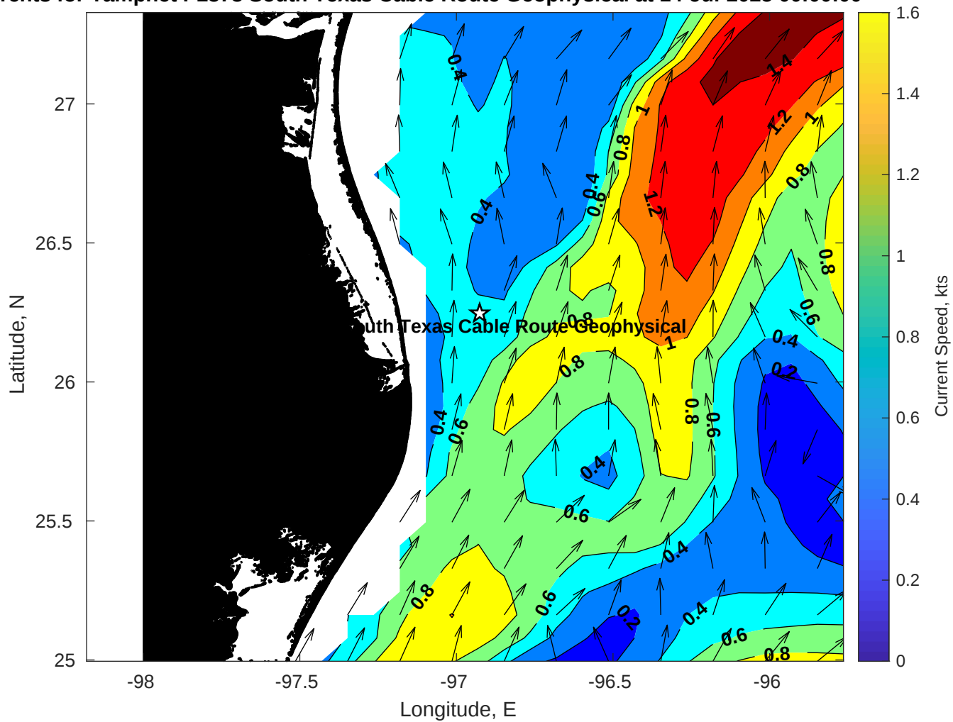
Surface Currents for Tampnet P2378 South Texas Cable Route Geophysical at 14-Jul-2025 00:00:00
