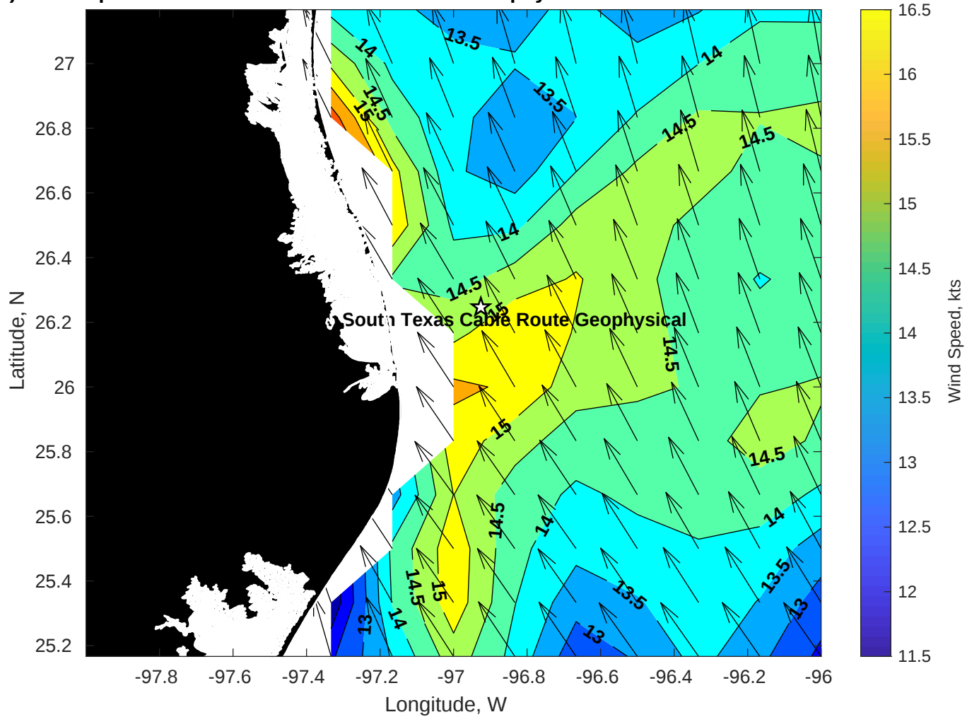
Winds (kts) for Tampnet P2378 South Texas Cable Route Geophysical at 15-Jul-2025 09:00:00
