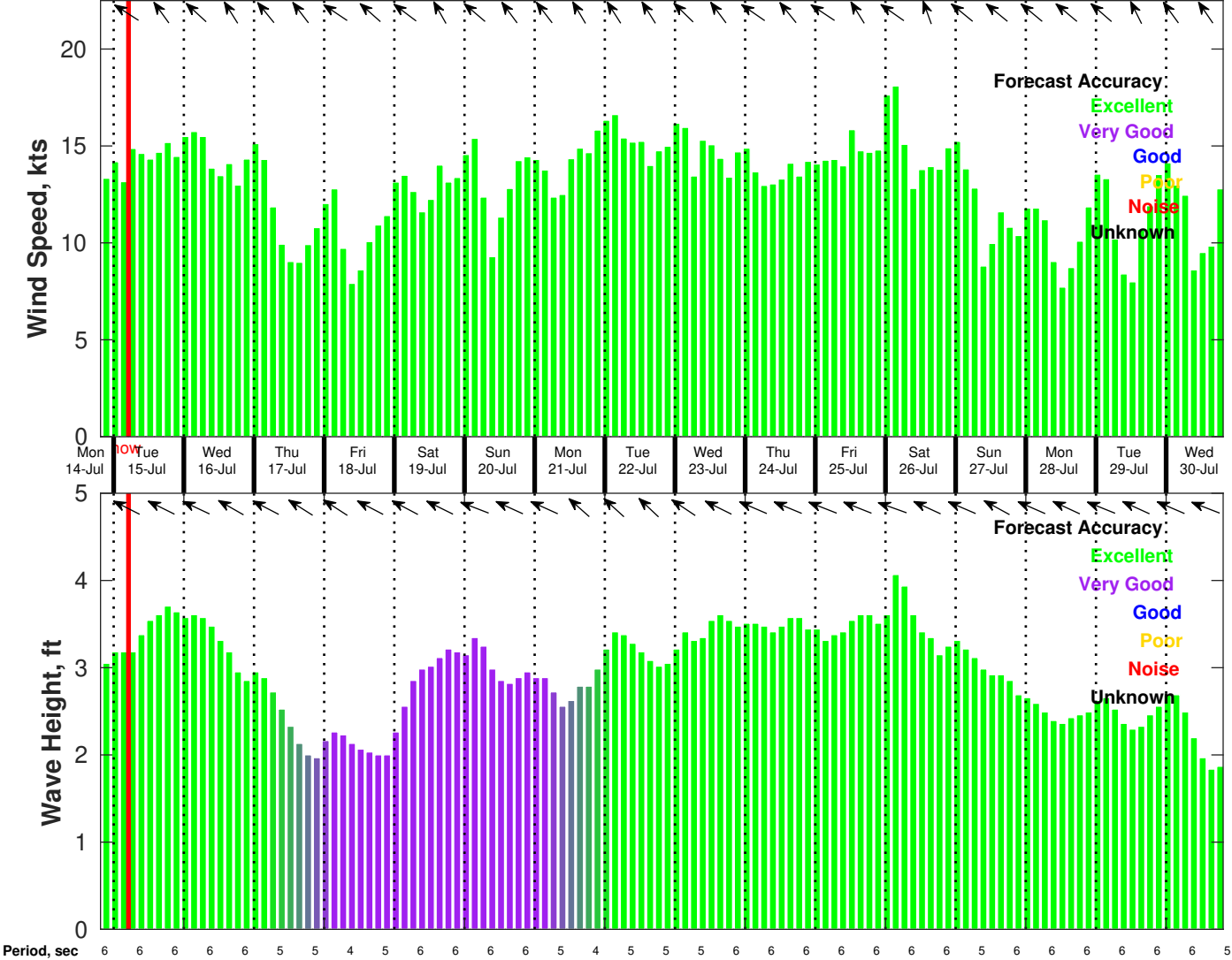
Wind & Wave Forecast for Tampnet P2378 South Texas Cable Route Geophysical from 14-Jul-2025 20:00:00 to 30-Jul-2025 20:00:00
