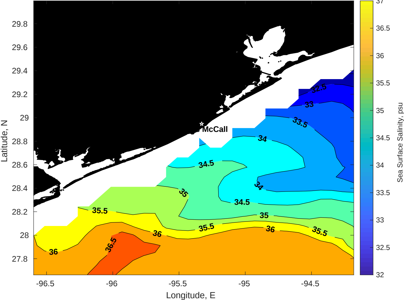
Surface Salinity for Brooks McCall at 15-Jul-2025 00:00:00
