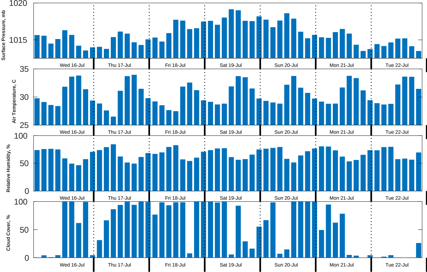
Met Forecast for Brooks McCall from 16-Jul-2025 00:00:00 to 23-Jul-2025 00:00:00
