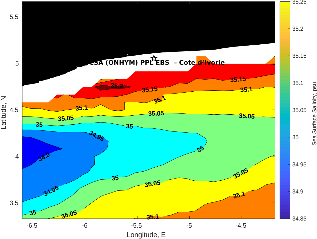
Surface Salinity for CSA (ONHYM) PPL EBS - Cote d'Ivoire at 15-Jul-2025 00:00:00
