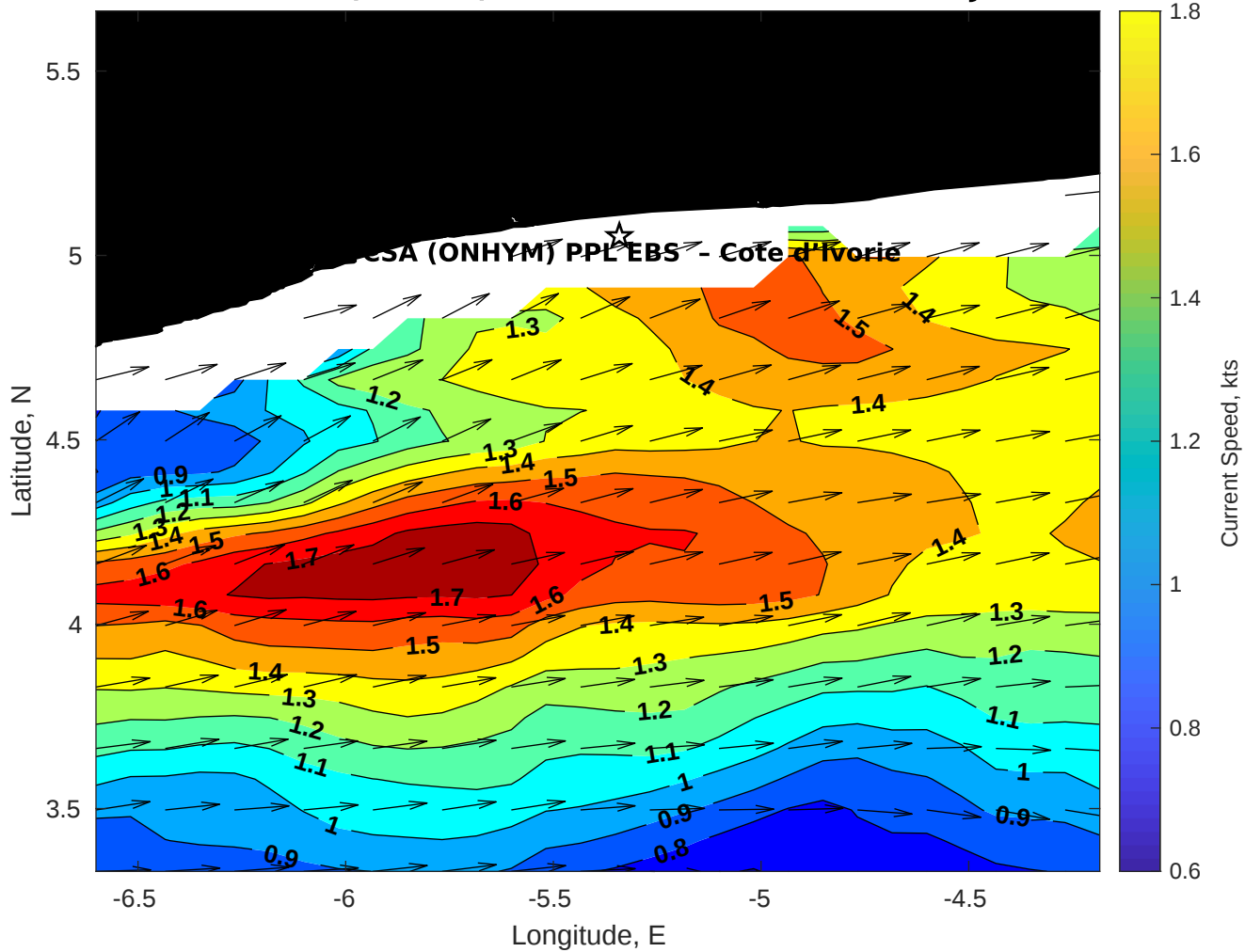
Surface Currents for CSA (ONHYM) PPL EBS - Cote d'Ivoire at 15-Jul-2025 00:00:00
