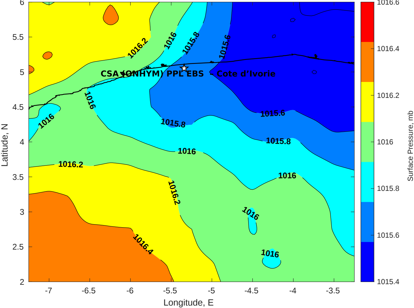
Surface Pressure (mb) for CSA (ONHYM) PPL EBS - Cote d'Ivoire at 17-Jul-2025 00:00:00
