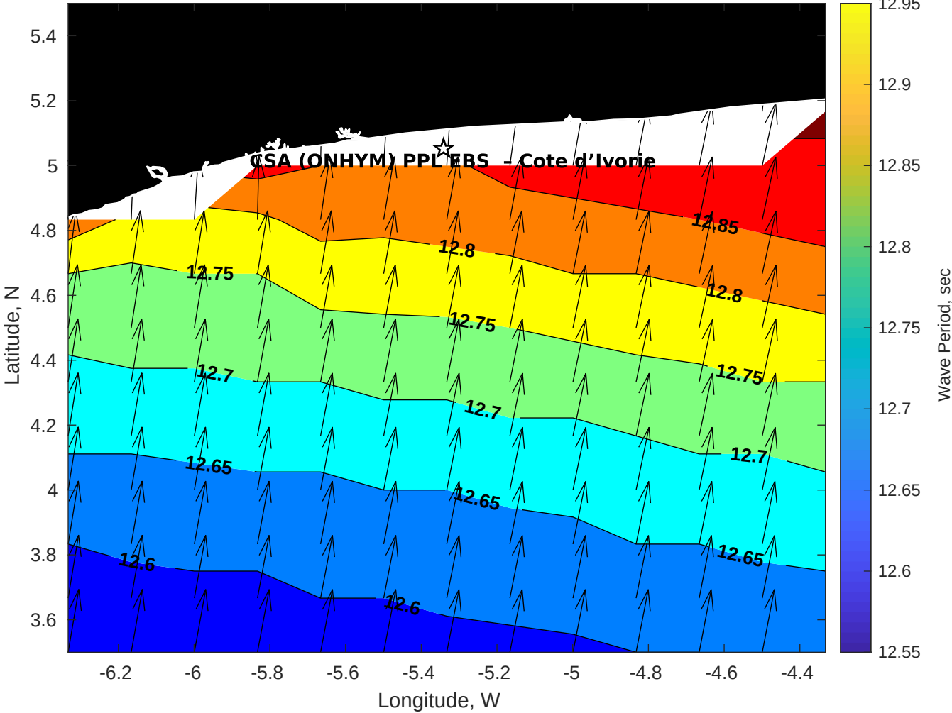
Wave Period (sec) for CSA (ONHYM) PPL EBS - Cote d'Ivoire at 16-Jul-2025 09:00:00
