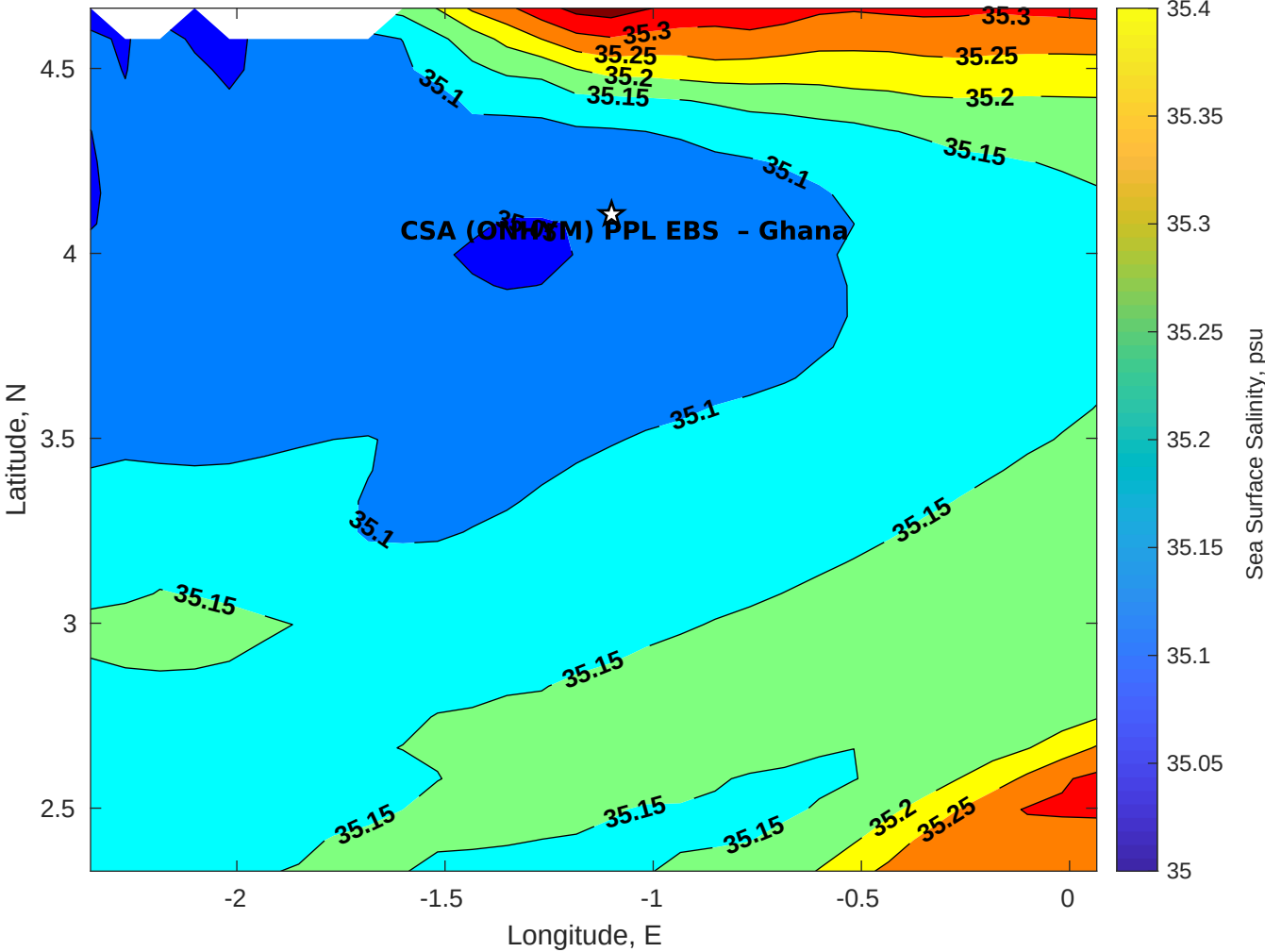
Surface Salinity for CSA (ONHYM) PPL EBS - Ghana at 15-Jul-2025 00:00:00
