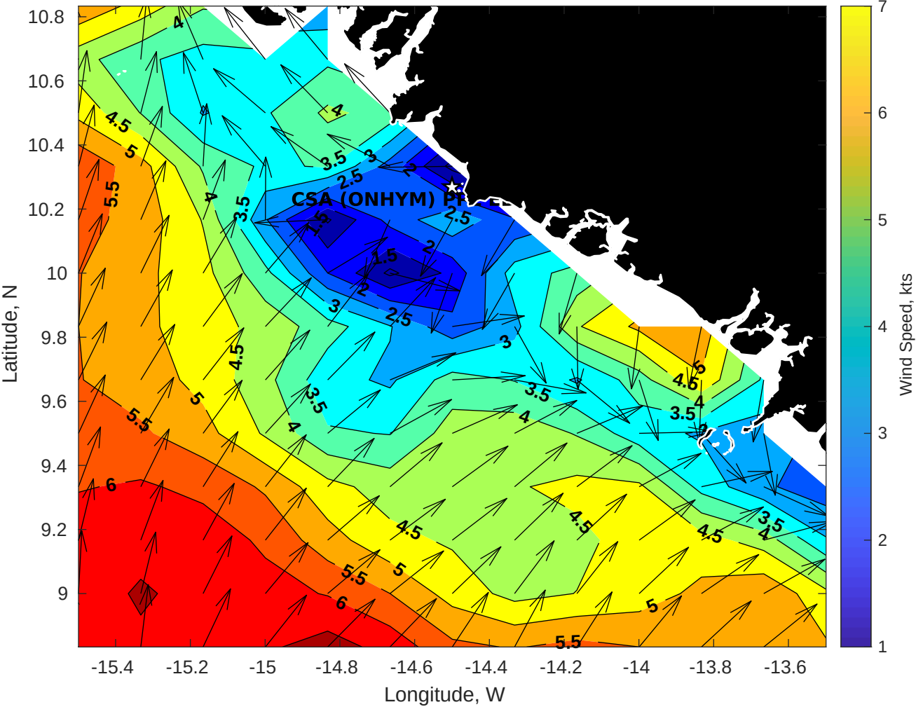
Winds (kts) for CSA (ONHYM) PPL EBS - Guinea at 16-Jul-2025 09:00:00
