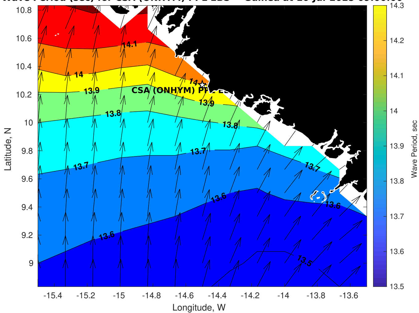
Wave Period (sec) for CSA (ONHYM) PPL EBS - Guinea at 16-Jul-2025 09:00:00
