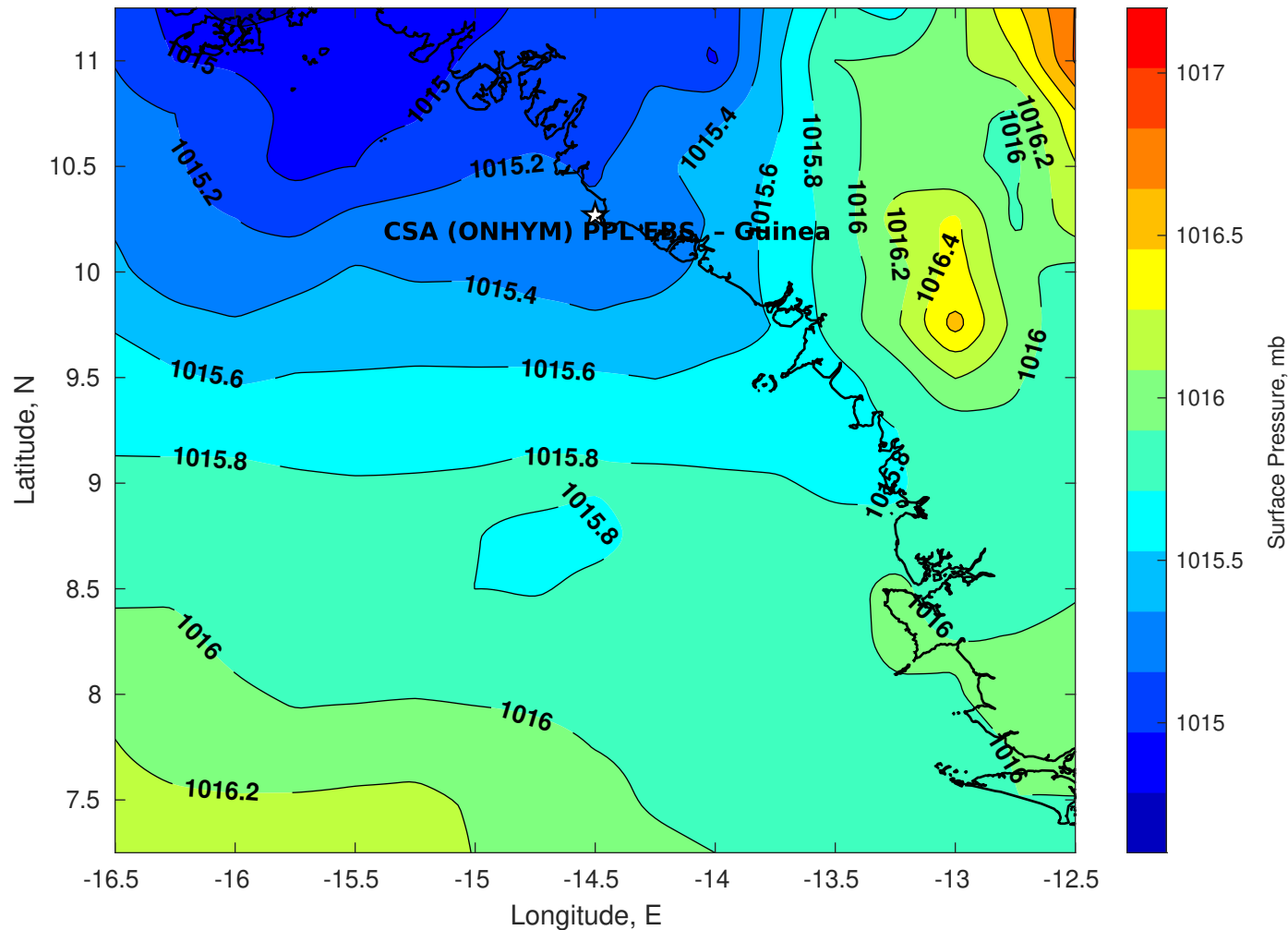
Surface Pressure (mb) for CSA (ONHYM) PPL EBS - Guinea at 18-Jul-2025 00:00:00
