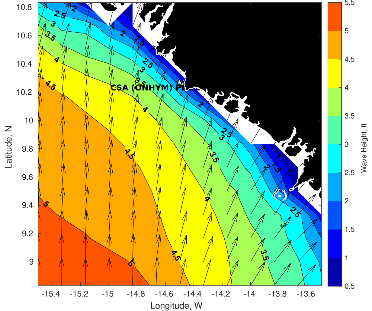
Wave Height (ft) for CSA (ONHYM) PPL EBS - Guinea at 16-Jul-2025 09:00:00
