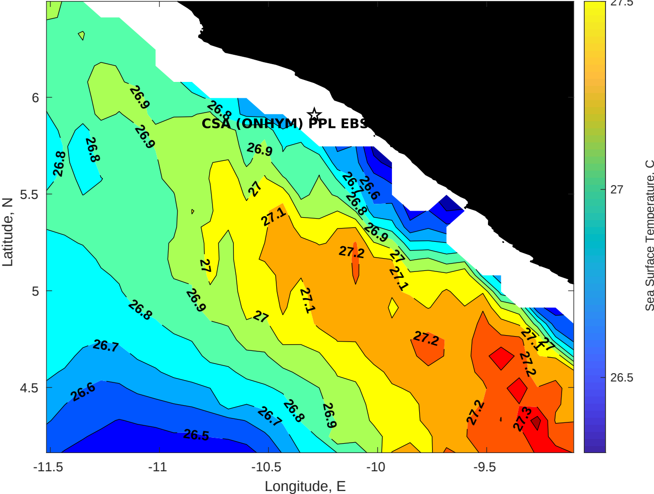
SST for CSA (ONHYM) PPL EBS - Liberia at 15-Jul-2025 00:00:00
