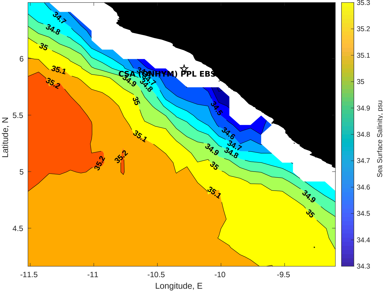
Surface Salinity for CSA (ONHYM) PPL EBS - Liberia at 15-Jul-2025 00:00:00
