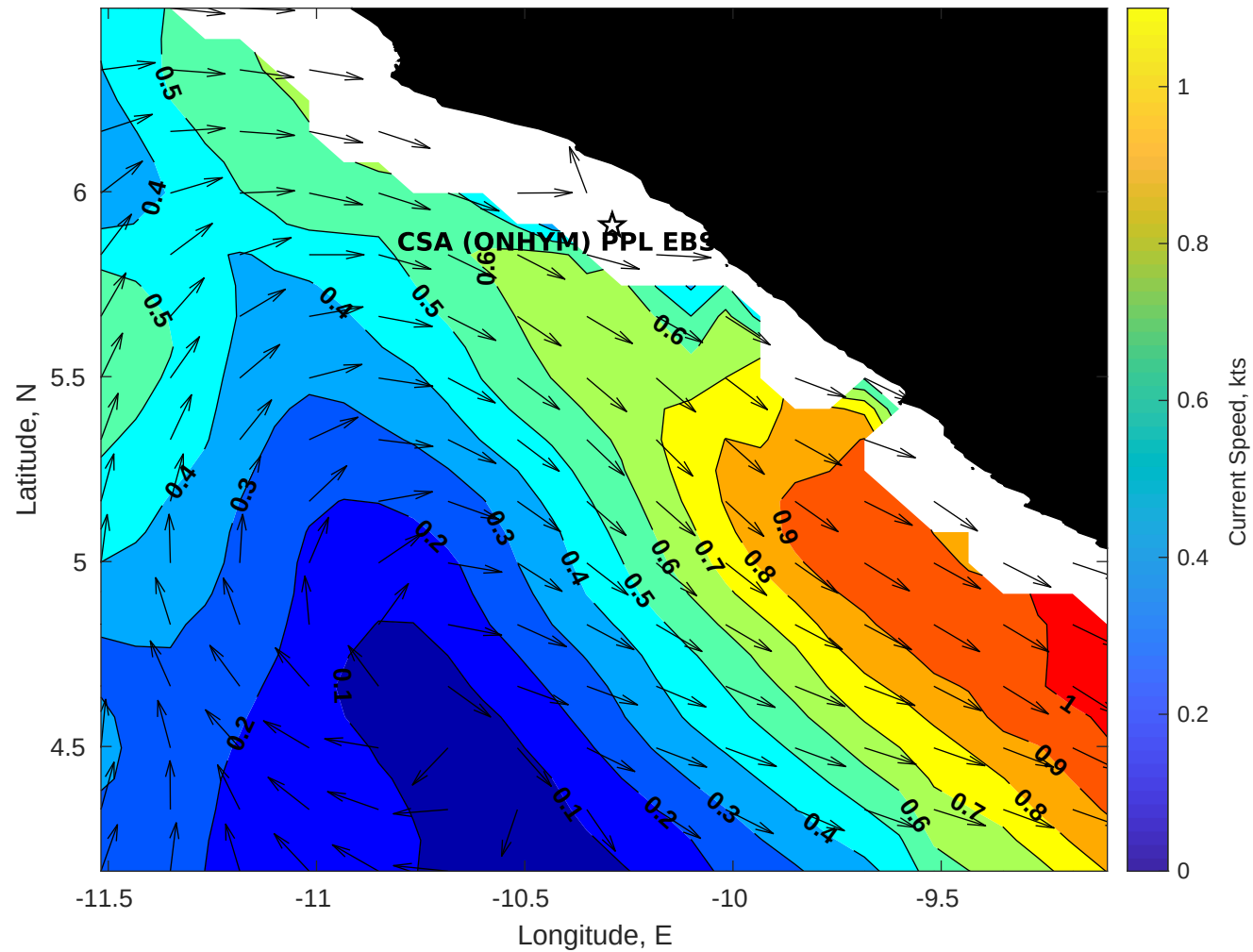
Surface Currents for CSA (ONHYM) PPL EBS - Liberia at 15-Jul-2025 00:00:00
