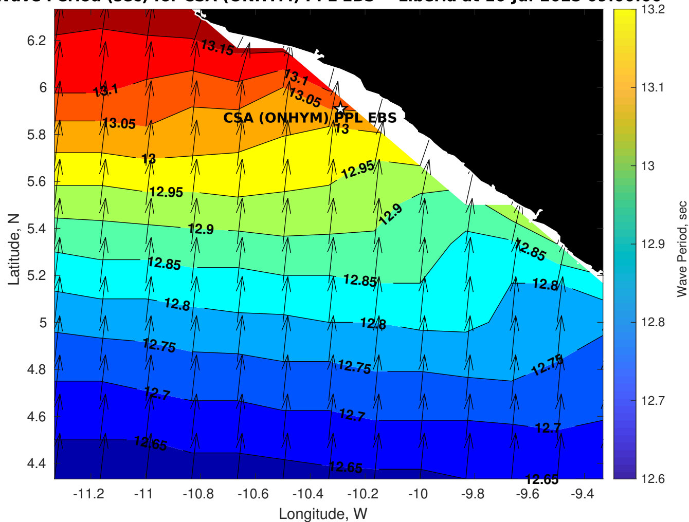
Wave Period (sec) for CSA (ONHYM) PPL EBS - Liberia at 16-Jul-2025 09:00:00
