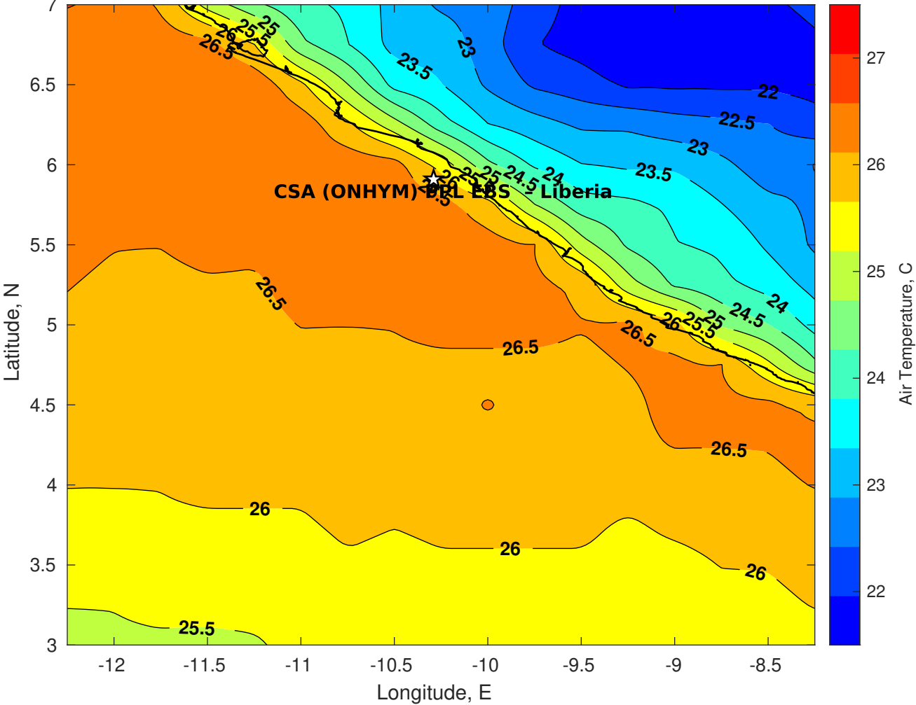
Air Temperature (C) for CSA (ONHYM) PPL EBS - Liberia at 16-Jul-2025
