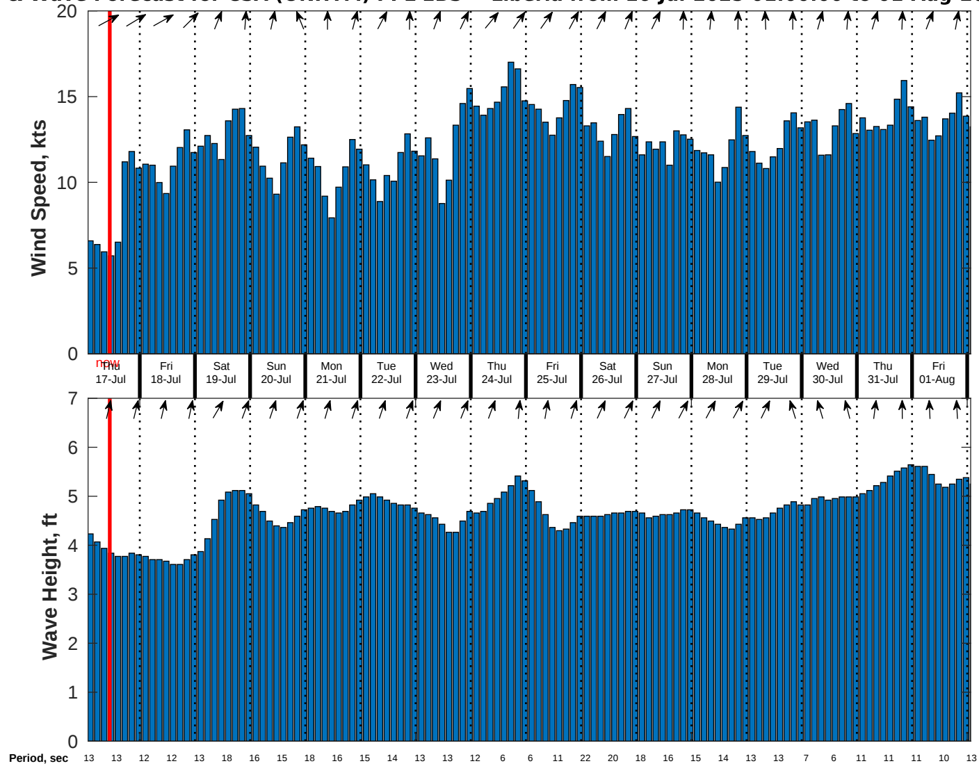
Wind & Wave Forecast for CSA (ONHYM) PPL EBS - Liberia from 16-Jul-2025 01:00:00 to 01-Aug-2025 01:00:00
