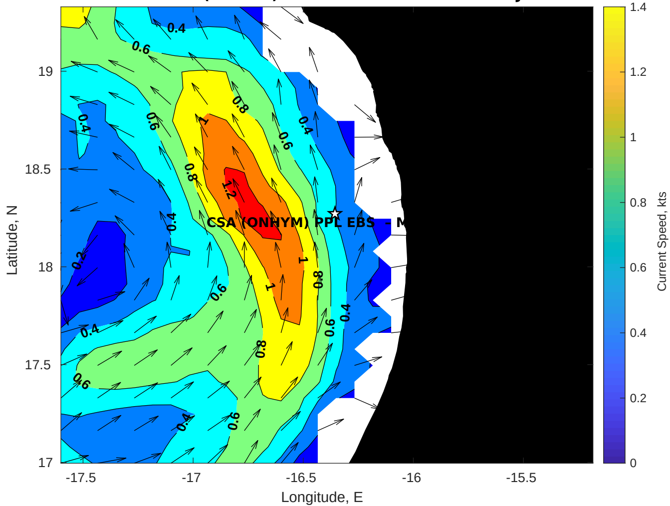
Surface Currents for CSA (ONHYM) PPL EBS - Mauritania at 15-Jul-2025 00:00:00
