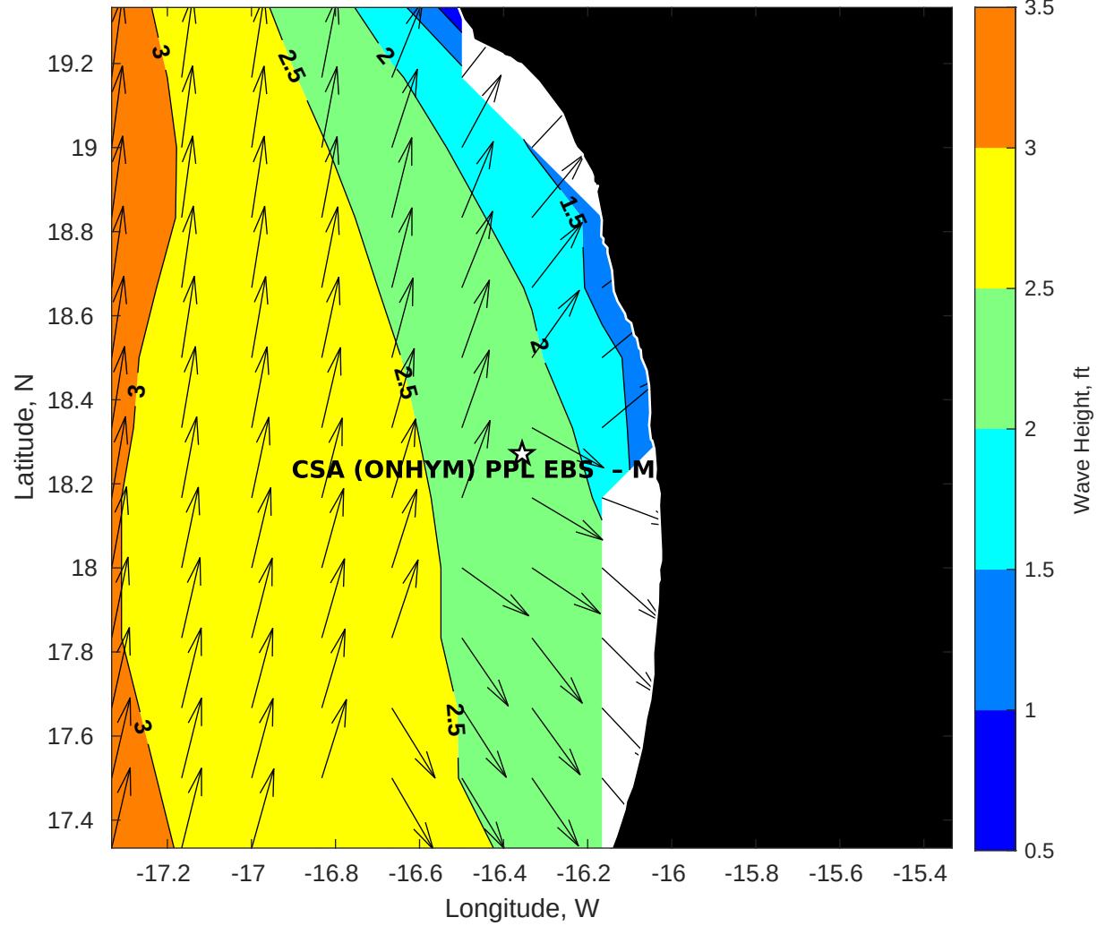
Wave Height (ft) for CSA (ONHYM) PPL EBS - Mauritania at 16-Jul-2025 09:00:00
