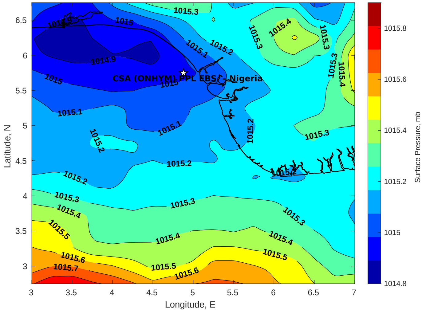
Surface Pressure (mb) for CSA (ONHYM) PPL EBS - Nigeria at 17-Jul-2025 00:00:00
