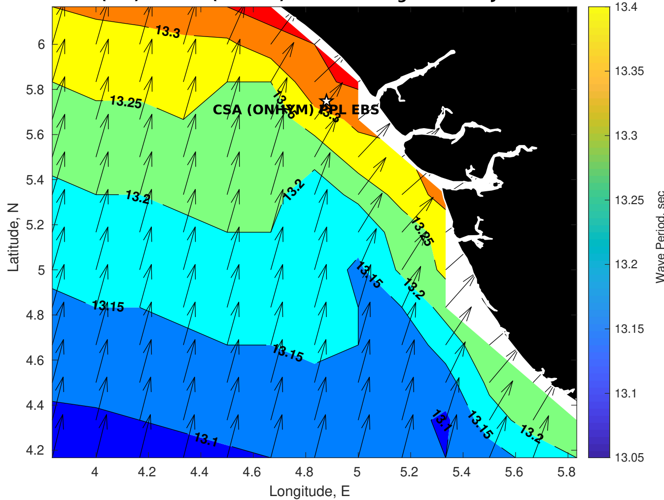
Wave Period (sec) for CSA (ONHYM) PPL EBS - Nigeria at 16-Jul-2025 09:00:00
