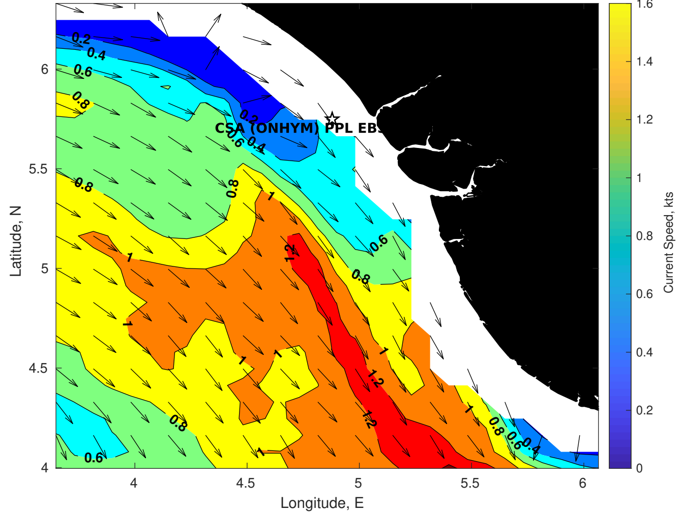
Surface Currents for CSA (ONHYM) PPL EBS - Nigeria at 15-Jul-2025 00:00:00
