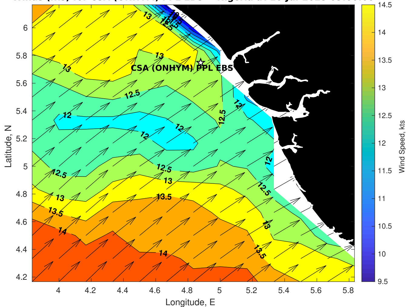
Winds (kts) for CSA (ONHYM) PPL EBS - Nigeria at 16-Jul-2025 09:00:00
