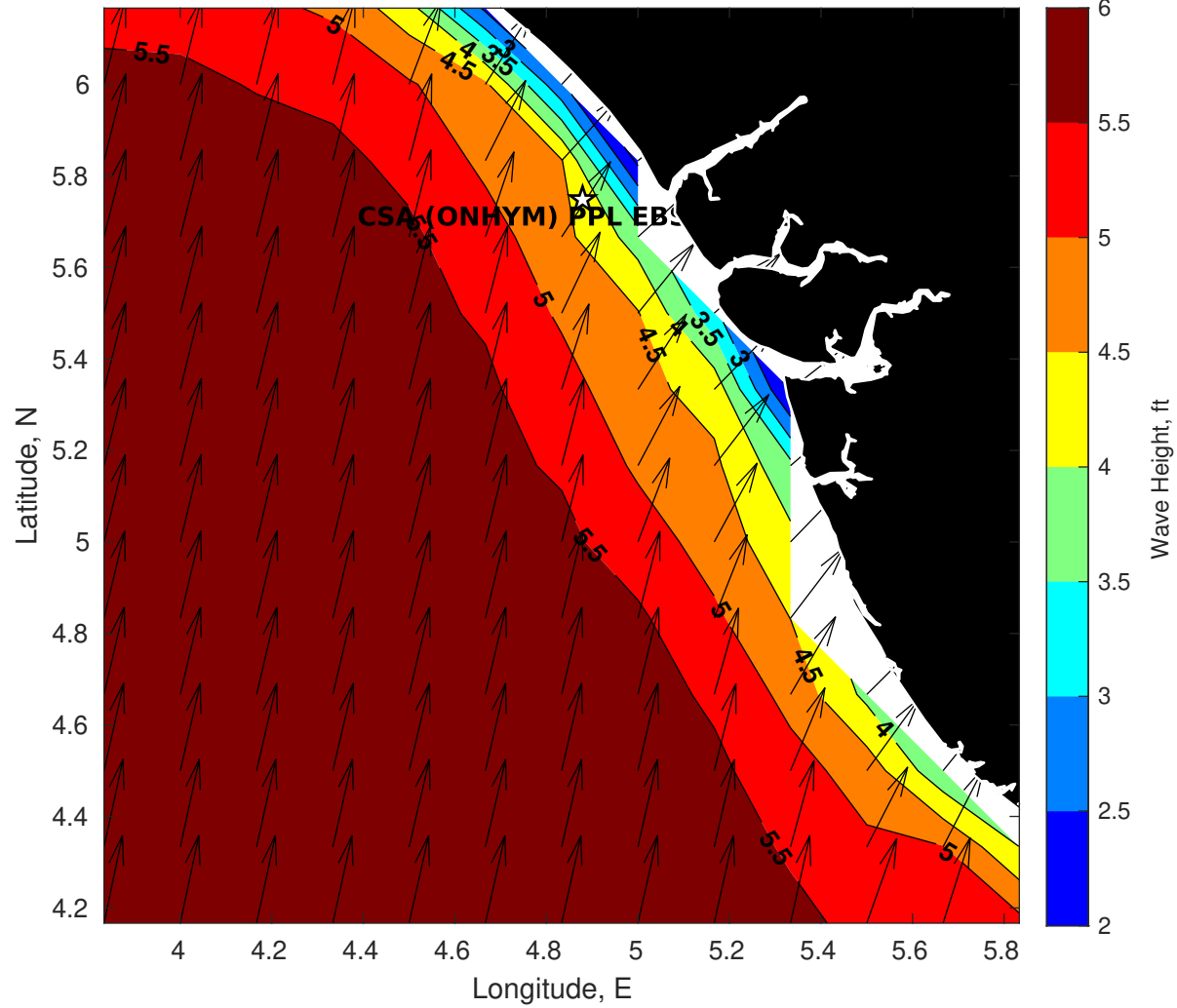
Wave Height (ft) for CSA (ONHYM) PPL EBS - Nigeria at 16-Jul-2025 09:00:00
