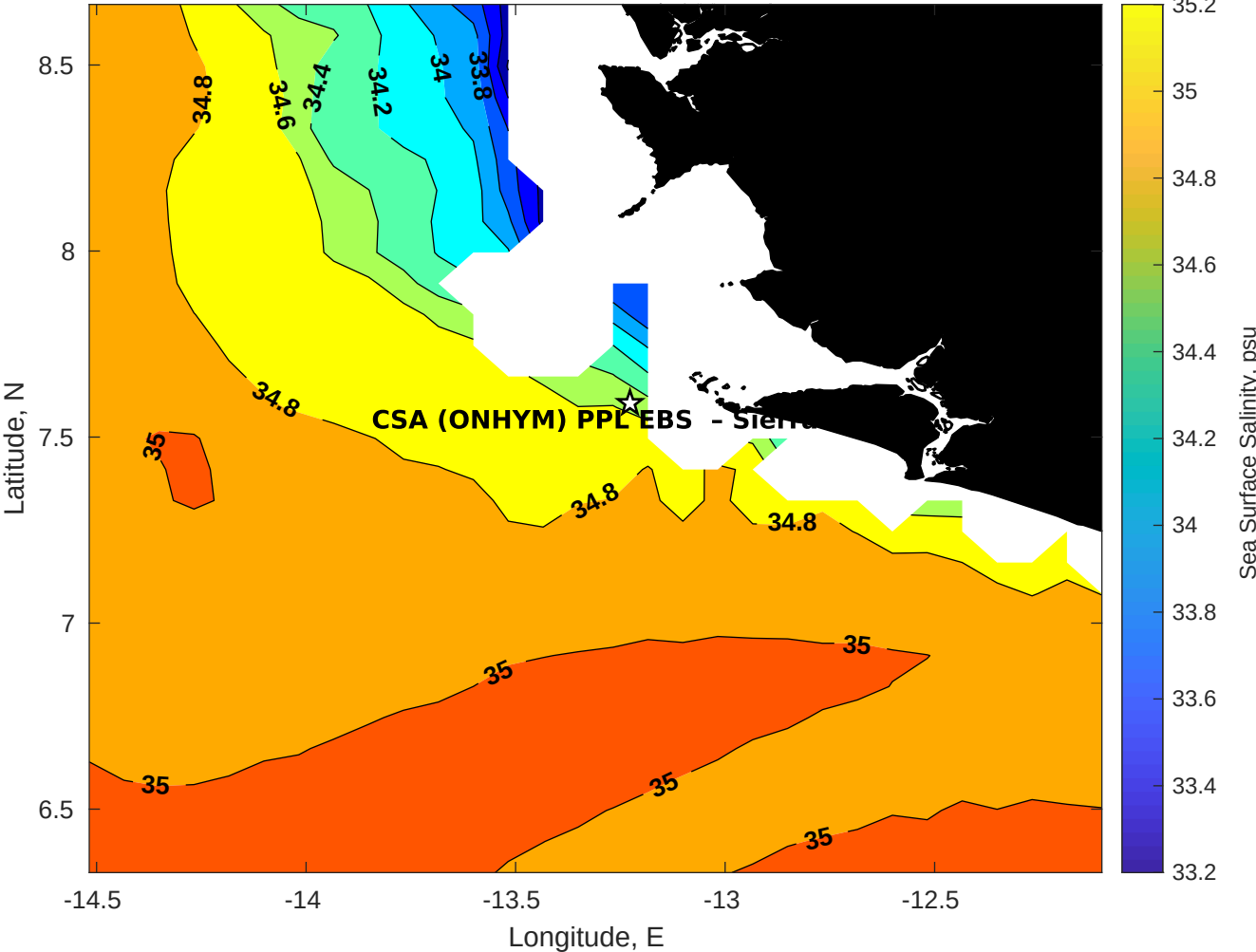
Surface Salinity for CSA (ONHYM) PPL EBS - Sierra Leone at 15-Jul-2025 00:00:00
