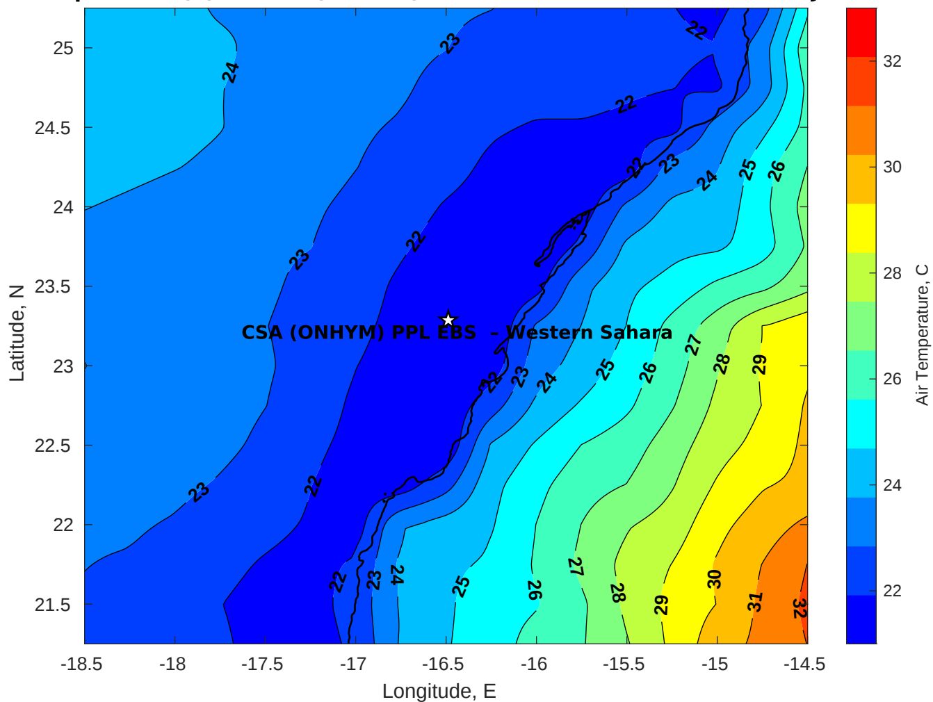
Air Temperature (C) for CSA (ONHYM) PPL EBS - Western Sahara at 16-Jul-2025
