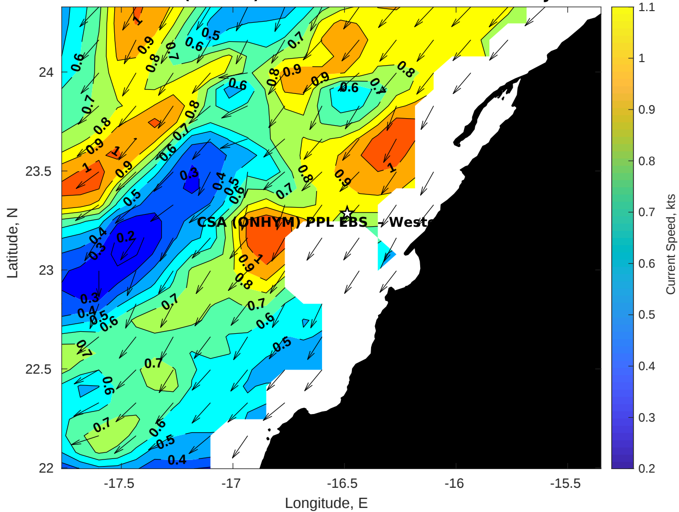
Surface Currents for CSA (ONHYM) PPL EBS - Western Sahara at 15-Jul-2025 00:00:00
