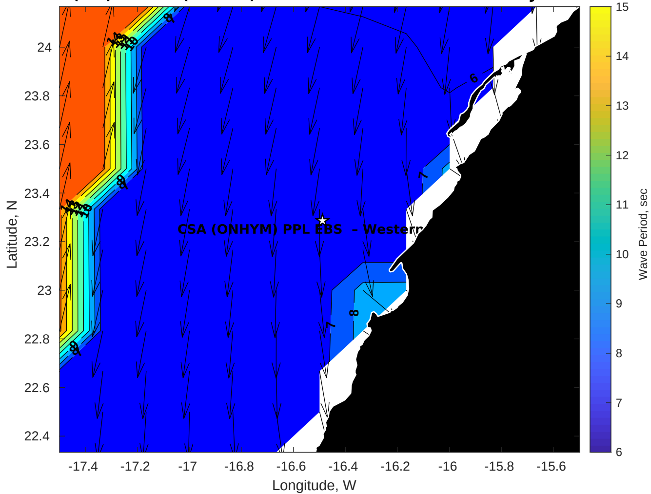
Wave Period (sec) for CSA (ONHYM) PPL EBS - Western Sahara at 16-Jul-2025 09:00:00
