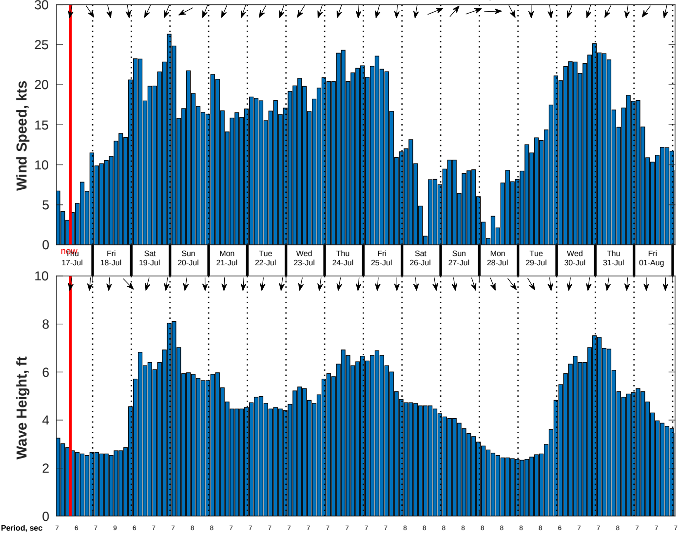
Wind & Wave Forecast for CSA (ONHYM) PPL EBS - Western Sahara from 16-Jul-2025 01:00:00 to 01-Aug-2025 01:00:00
