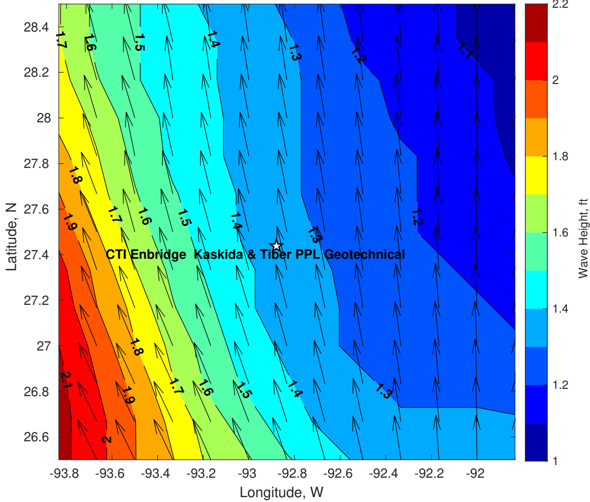
Wave Height (ft) for CTI Enbridge Kaskida & Tiber PPL Geotechnical at 16-Jul-2025 09:00:00
