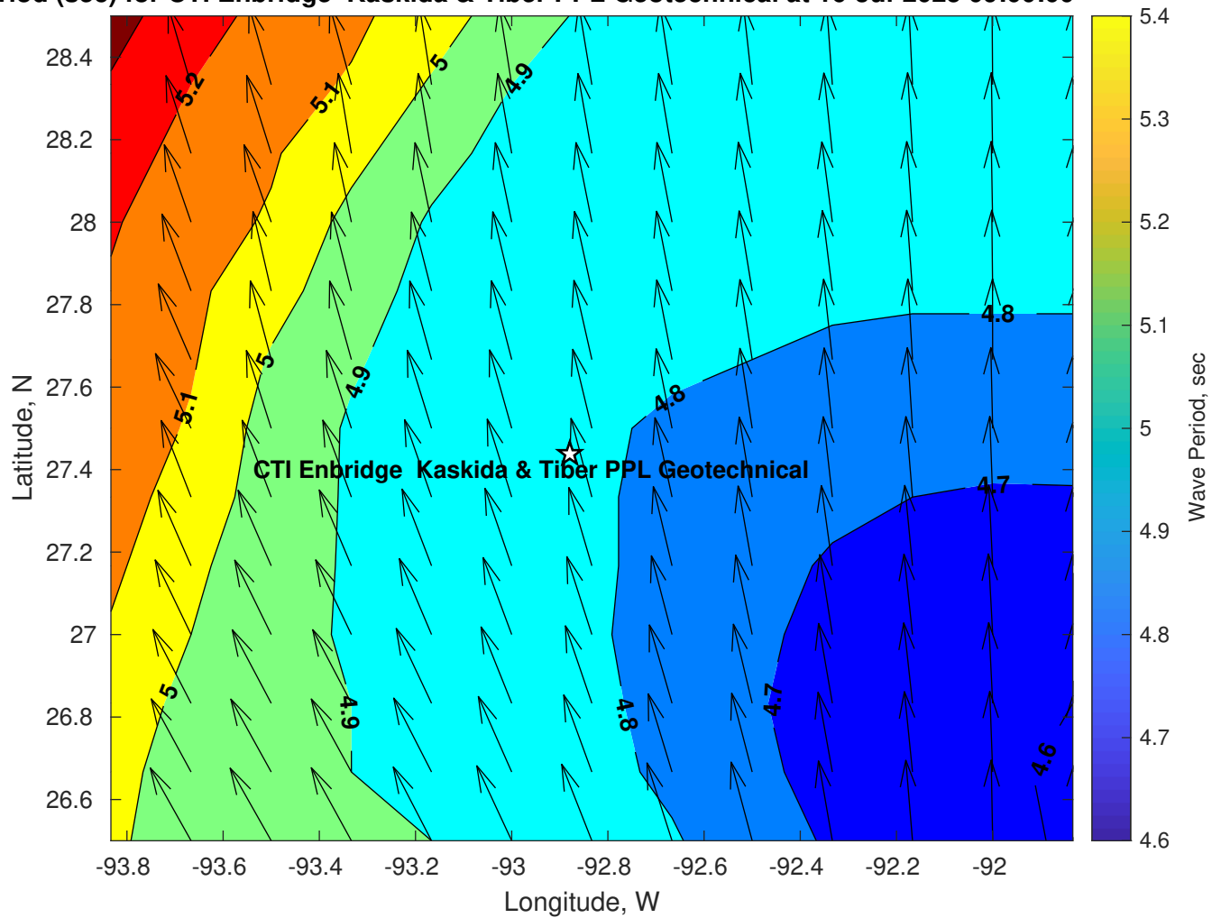
Wave Period (sec) for CTI Enbridge Kaskida & Tiber PPL Geotechnical at 16-Jul-2025 09:00:00
