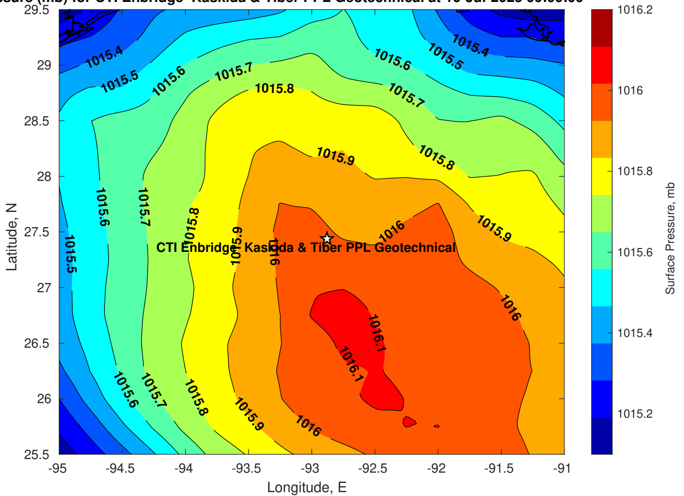
Surface Pressure (mb) for CTI Enbridge Kaskida & Tiber PPL Geotechnical at 16-Jul-2025 00:00:00
