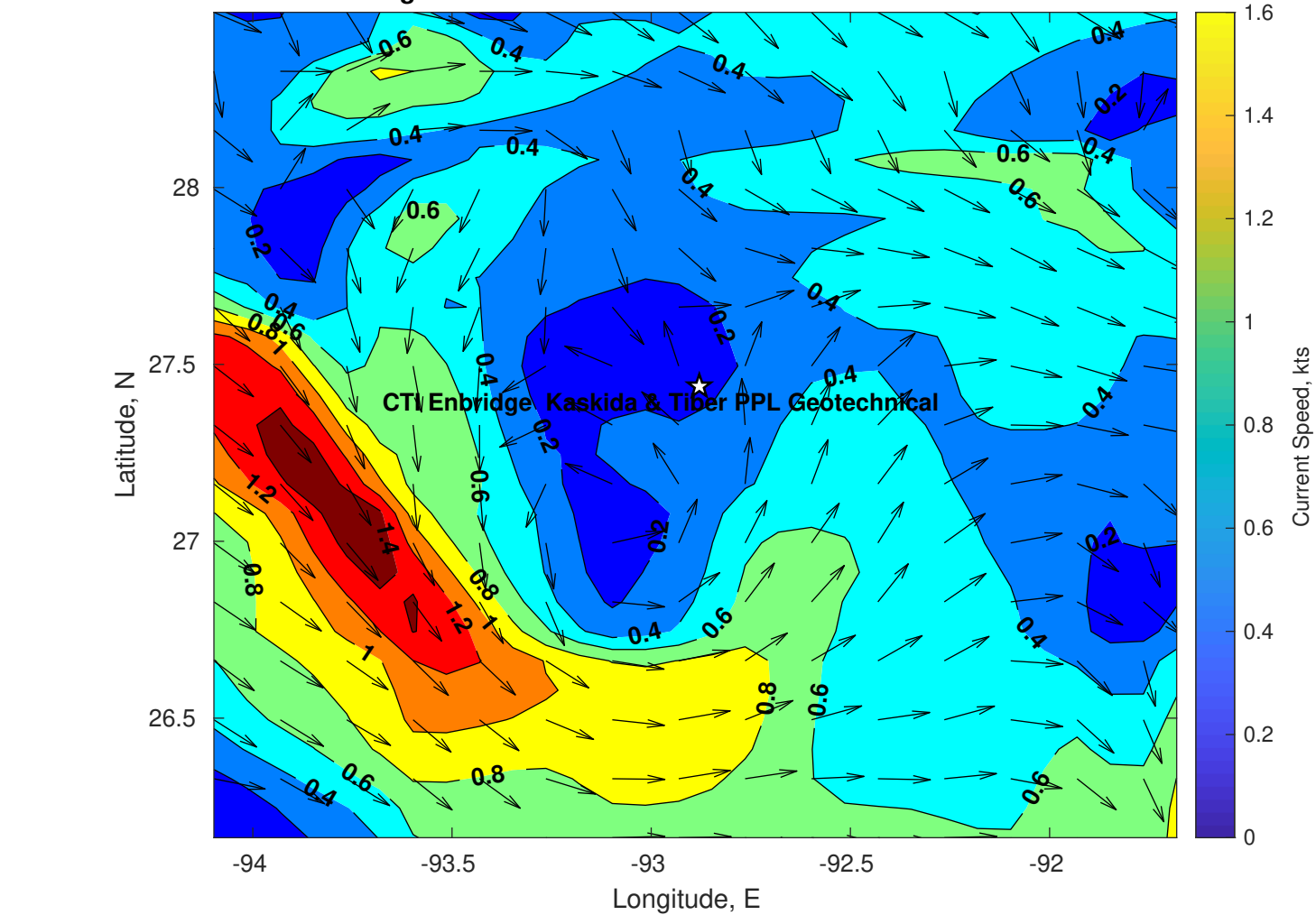
Surface Currents for CTI Enbridge Kaskida & Tiber PPL Geotechnical at 15-Jul-2025 00:00:00
