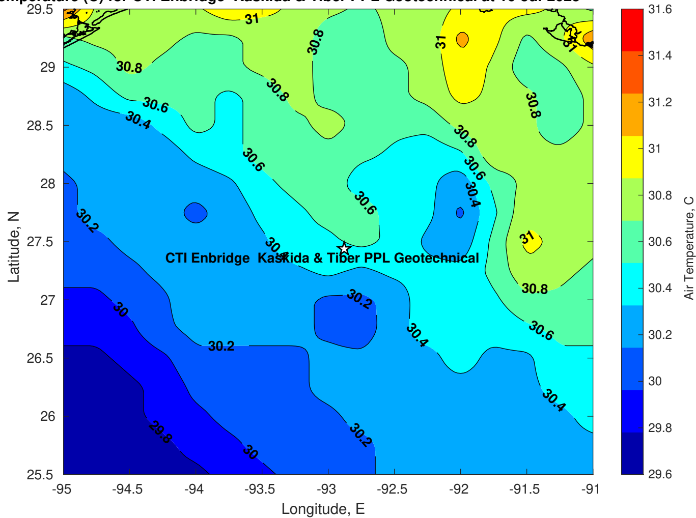
Air Temperature (C) for CTI Enbridge Kaskida & Tiber PPL Geotechnical at 16-Jul-2025
