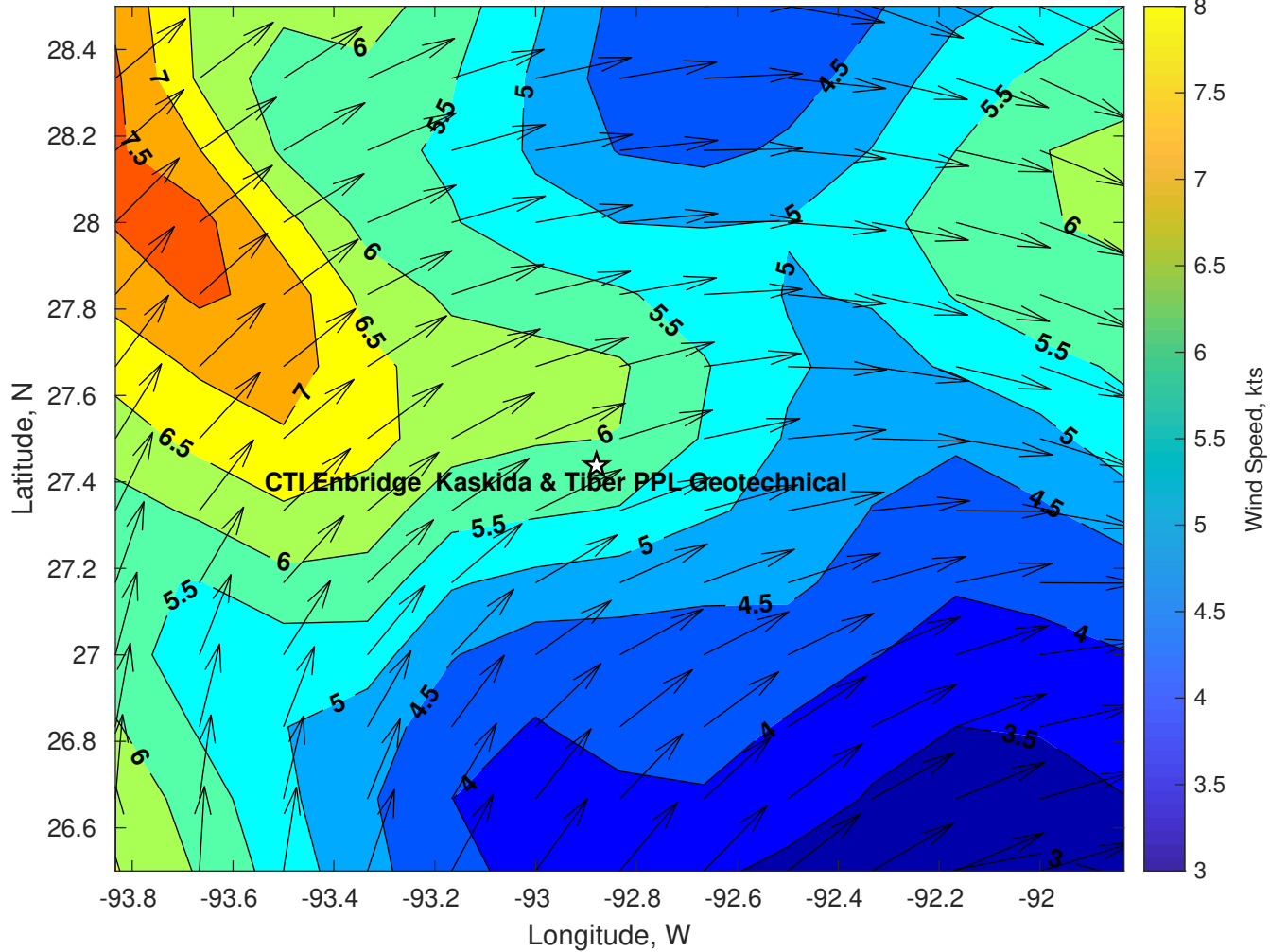
Winds (kts) for CTI Enbridge Kaskida & Tiber PPL Geotechnical at 16-Jul-2025 09:00:00
