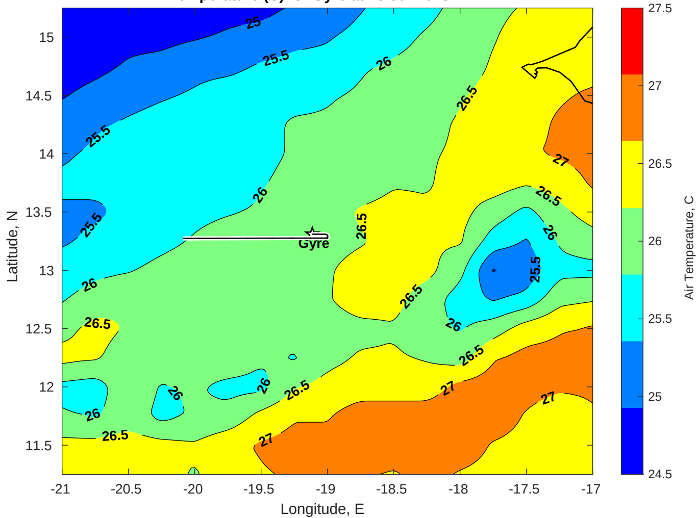
Air Temperature (C) for Gyre at 16-Jul-2025
