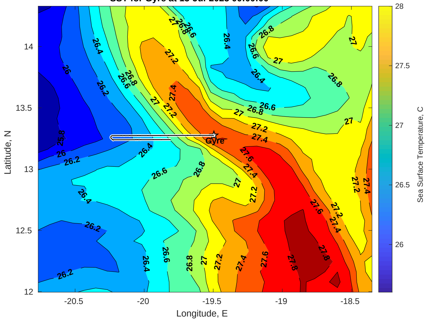
SST for Gyre at 15-Jul-2025 00:00:00
