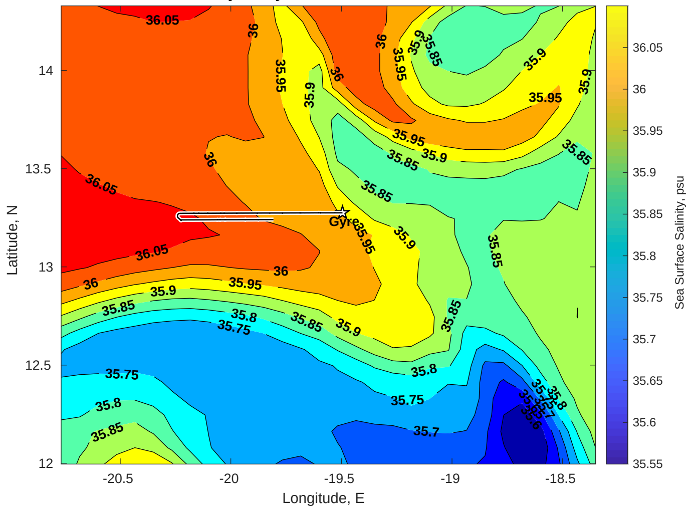
Surface Salinity for Gyre at 15-Jul-2025 00:00:00
