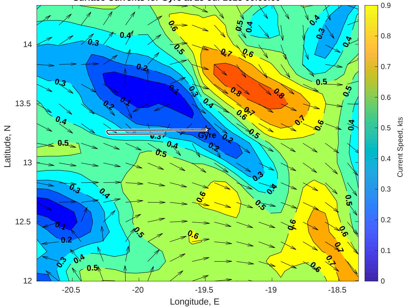
Surface Currents for Gyre at 15-Jul-2025 00:00:00
