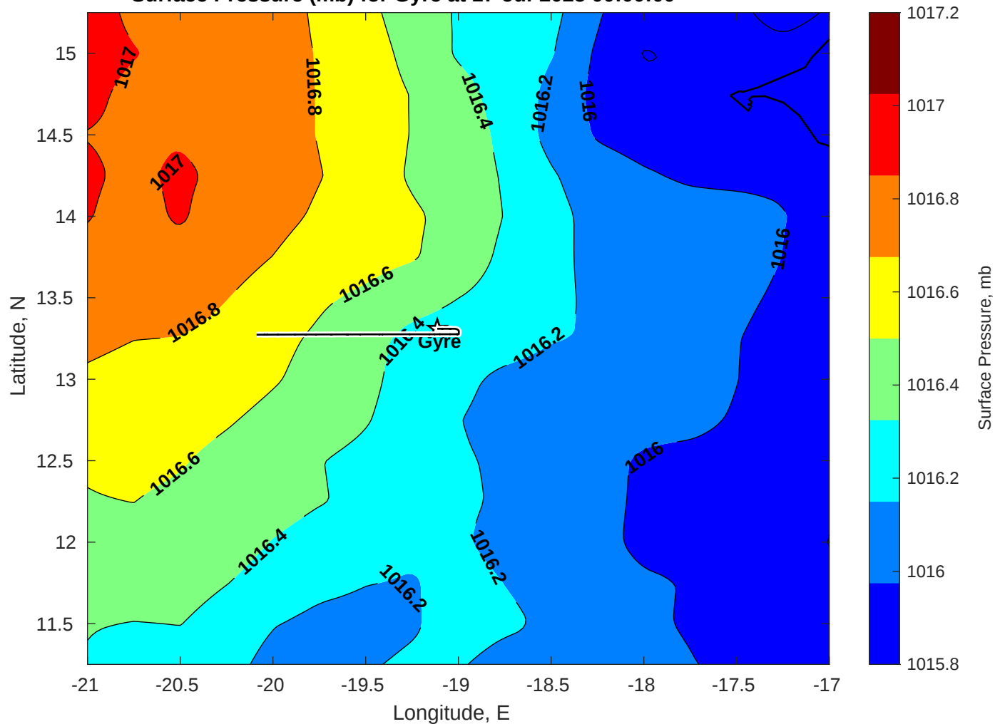
Surface Pressure (mb) for Gyre at 17-Jul-2025 00:00:00
