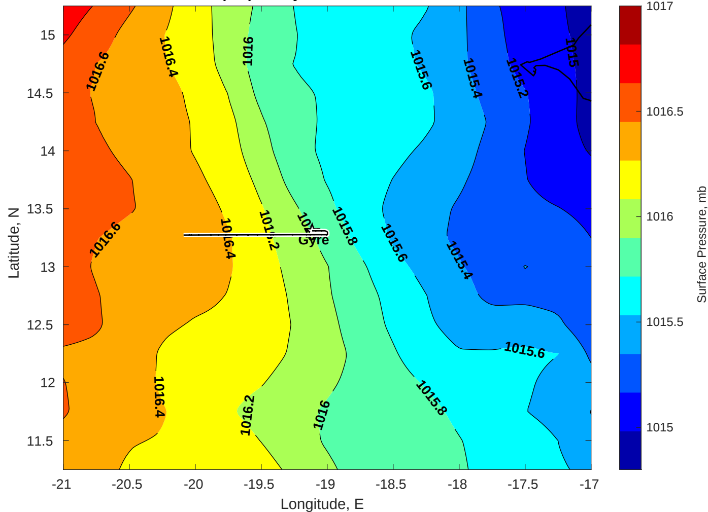
Surface Pressure (mb) for Gyre at 18-Jul-2025 00:00:00
