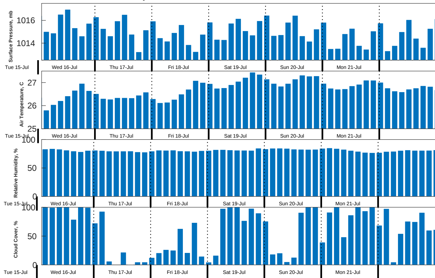
Met Forecast for Gyre from 15-Jul-2025 23:00:00 to 22-Jul-2025 23:00:00
